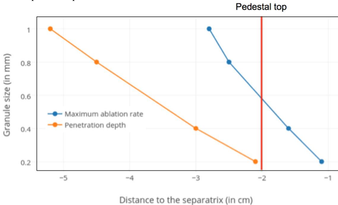
FIG. 4. Positions where the granules are at maximum ablation and where the granules are completely ablated, for different granule initial sizes and a velocity of 100 m/s. Distance is given in cm inside the separatrix (at r = 0 cm) and the position of the pedestal top (at r = -2 cm) is given.
