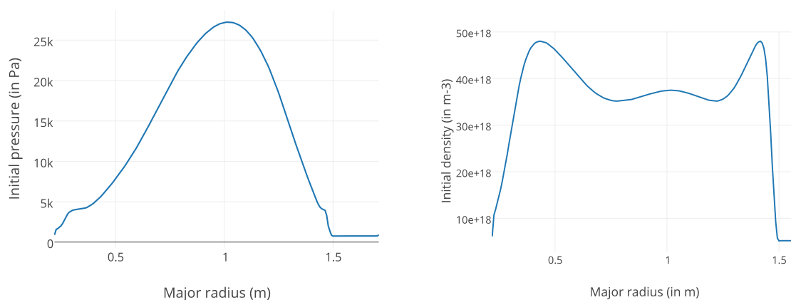
FIG. 1. Initial NSTX pressure and density profiles (before firing a Lithium Granule). These are experimental profiles within an inter-ELM time interval.
