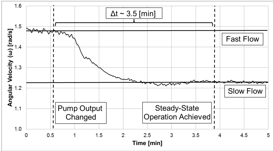
Figure 10 – The transient response of the RLFF used in this paper experiencing a sudden change in flow. Experimental data was averaged over a 10 [sec] interval to produce this plot.
