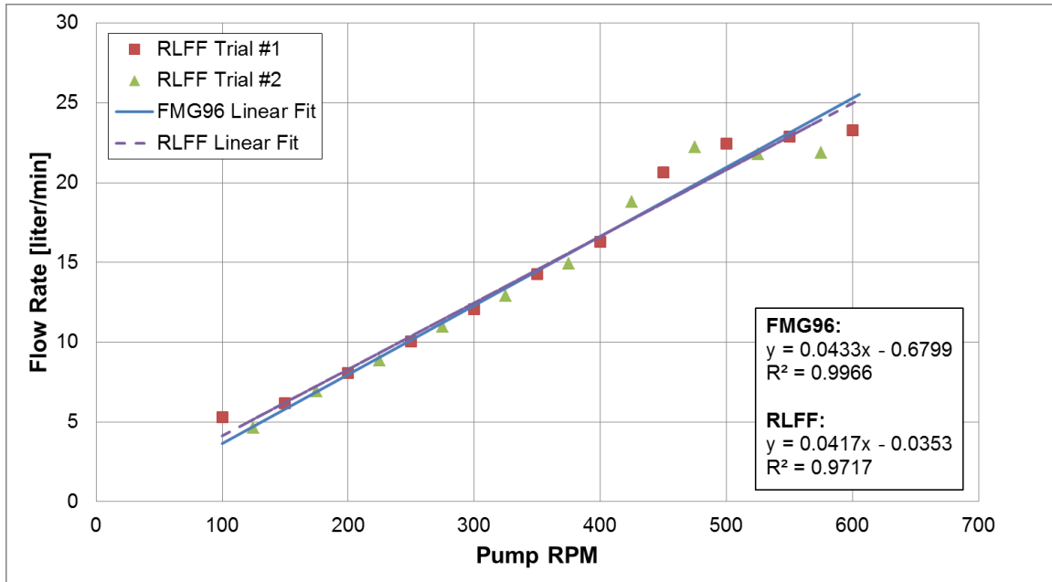
Figure 9 - Results of the intermittently operating RLFF compared to the linear fit of the FMG96 data. The average error of all data points on this plot is approximately 6%.
