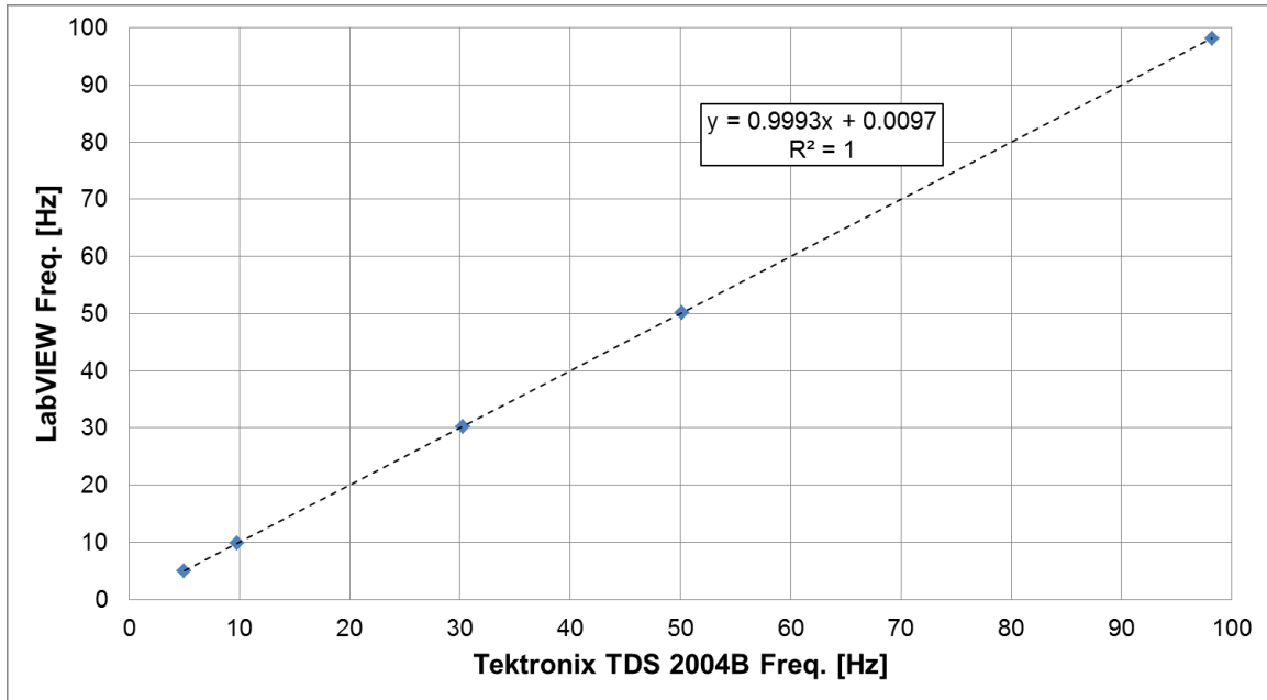
Figure 11 - Comparison of frequency measurements performed using the LabVIEW data acquisition setup and a Tektronix oscilloscope. The two devices yielded effectively identical results which demonstrated that the DAQ was functioning properly. The LabVIEW system sampled at a rate of 119-250 [kHz].
