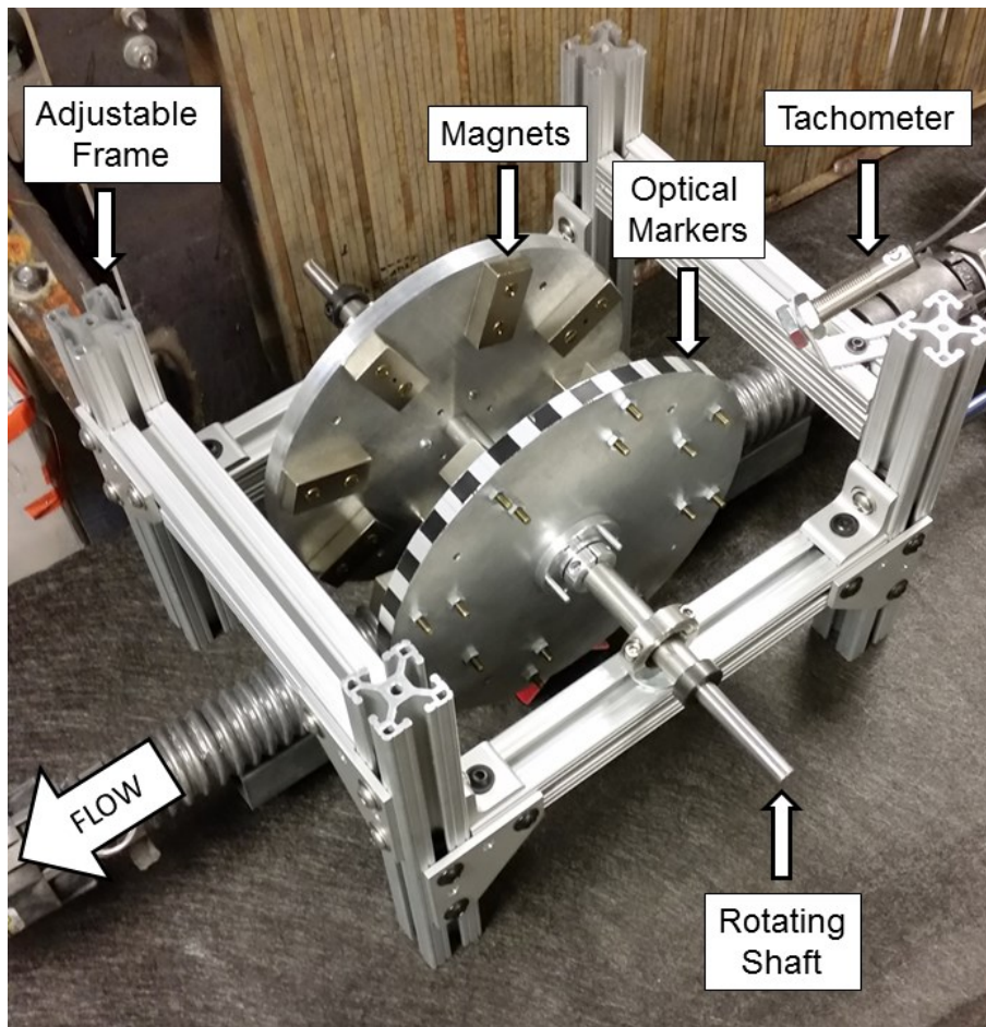
Figure 5 – A photo of the rotating Lorentz-force flowmeter used in this experiment.
