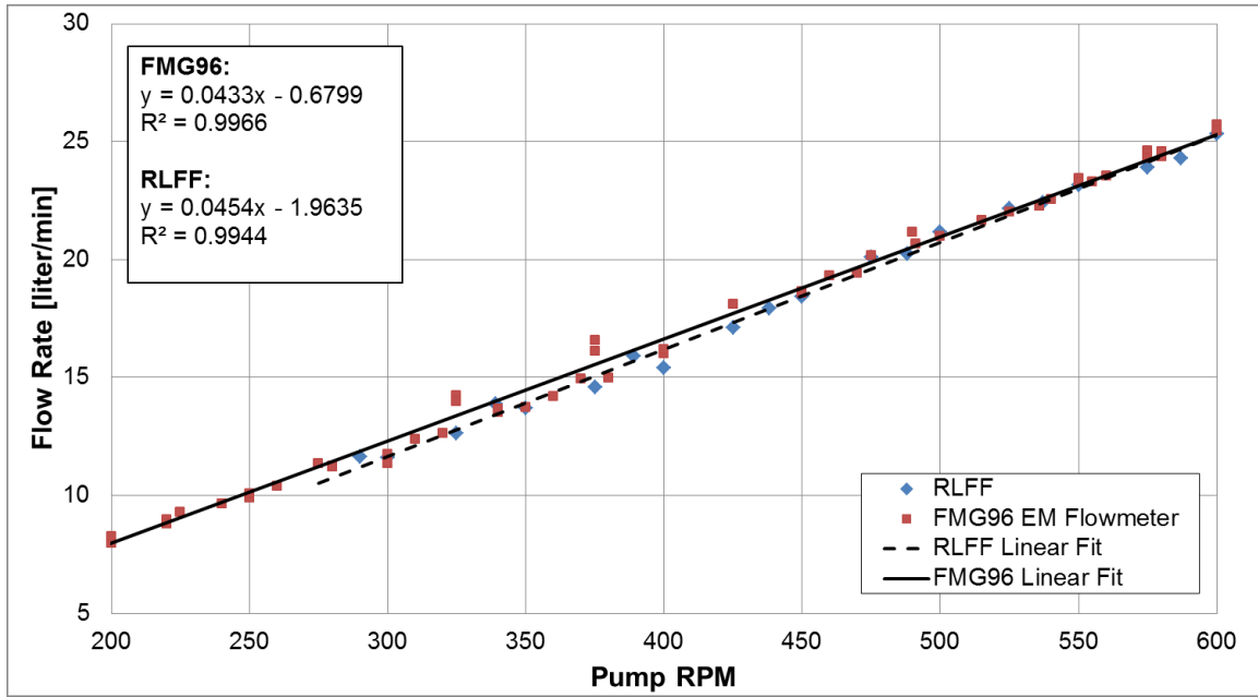
Figure 8 – A comparison of the FMG96 and the continuously operating RLFF measurements. The slopes of the linear fits agree to within < 5% difference.
