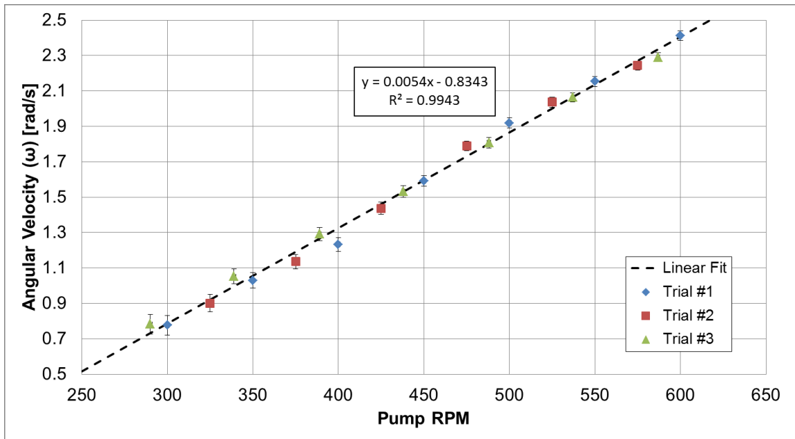
Figure 7 – Angular velocity data collected from the continuously operating RLFF.
