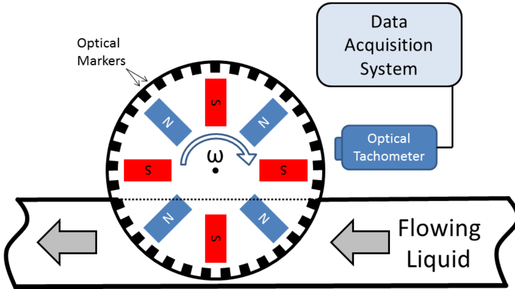
Figure 1 – A simple depiction of a Lorentz-force flowmeter setup. The magnet assembly is rimmed with multiple reflective services to enhance data collection. During operation, the magnet assembly rotates about a low-friction bearing located in the center of the disc.
