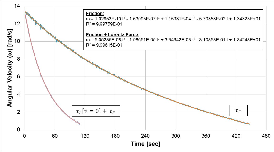
Figure 2 – A comparison of the flowmeter deceleration caused by either frictional forces or a combination of both frictional and Lorentz forces. The presence of the stagnant liquid metal had a pronounced impact on the deceleration of the rotating flowmeter. As shown above, all data can be accurately modeled using 4 th -order polynomial fits. The polynomial fits are only valid for the range of data shown in the plot.
