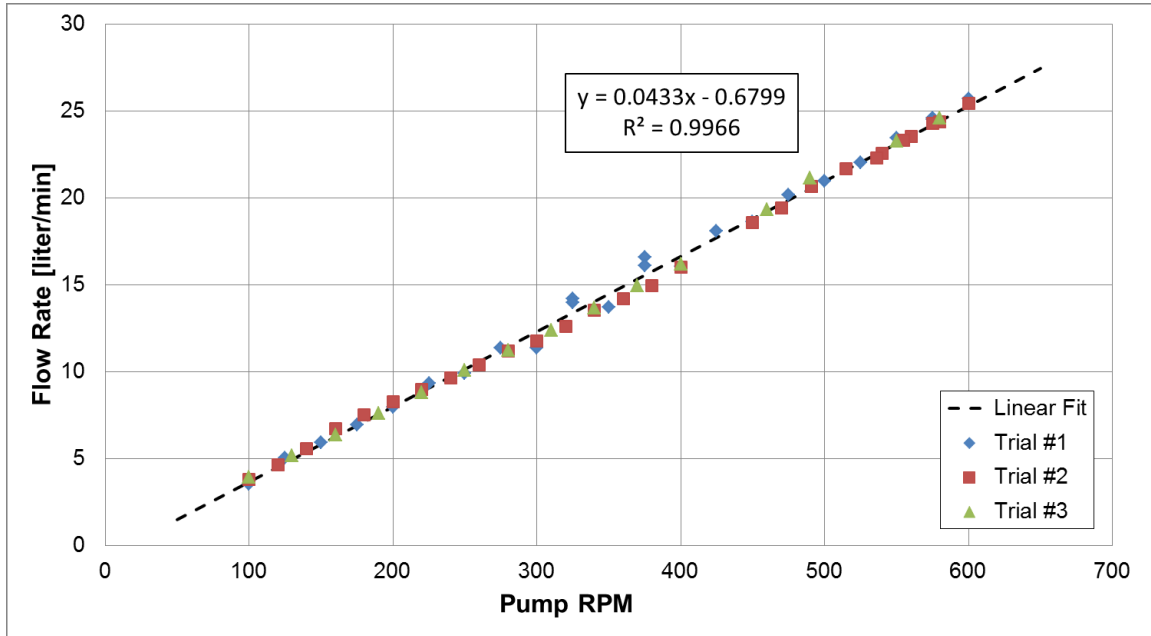
Figure 6 – The output of the gear-pump used in LMX. The galinstan flow rate as measured by the Omega FMG96 electromagnetic flowmeter. Error bars are not shown in this plot because they fall within the data markers.
