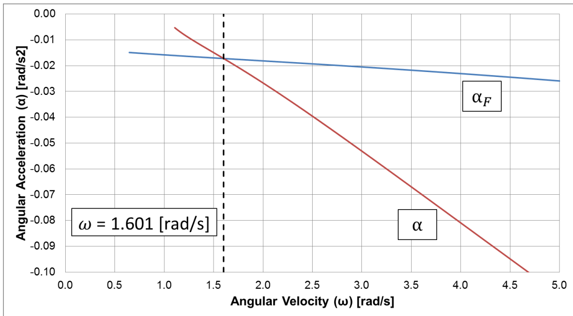
Figure 4 – Experimental data showing the intersection of the \alpha and \alpha_F plots. For this plot the pump operated at 300 revolutions per minute (RPM). It was determined that the two plots intersected at \omega = 1.601 [rad/s].
