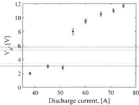
Fig. 10. Variation of the anode voltage drop with the discharge current.
