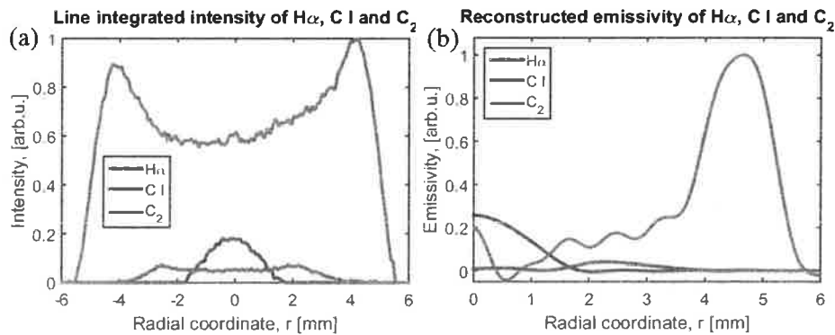
Fig. 4. (a) Radial profiles of line-integrated radiation intensity from Fig. 3 taken in the middle of the inter-electrode gap, (b) reconstruction of emissivity for each selected species in (a) for positive radial coordinates.
