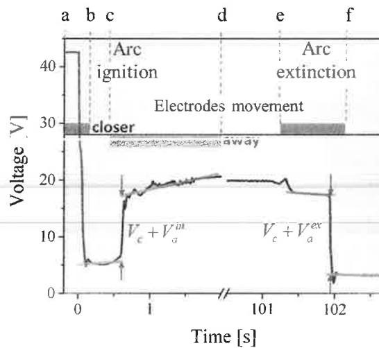
Fig. 9. Description of the anode fall and cathode fall measurements. Discharge voltage waveform (blue line) shown during arc ignition (a-d) and extinction (e-f). Electrodes are moving towards each other during (a-b) and (e-f) and outwards during (c-d). Red arrows indicate measurement points.
