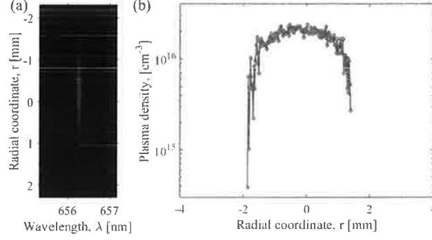
Fig. 8. (a) Spectral image of H_{\alpha} used to calculate (b) radial density profile, n_e(r) , in high ablation mode (20 V, 65 A, C9-A6).
