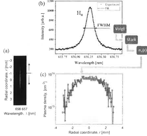
Fig. 7. Schematic of radial plasma density calculation using spectral image of H_{\alpha} (a) from the middle of the inter-electrode gap: horizontal slice of spectral image reveals spectral line profile (b) which is further de-convolved to obtain Stark broadening and n_e(r) at given radial coordinate. The result is a radial density profile, n_e(r) (c). (Low ablation mode, 21 V, 55 A, C9-A6).
