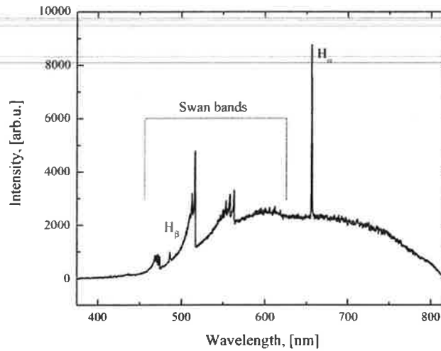
Fig. 3. Typical low-resolution arc spectrum.
