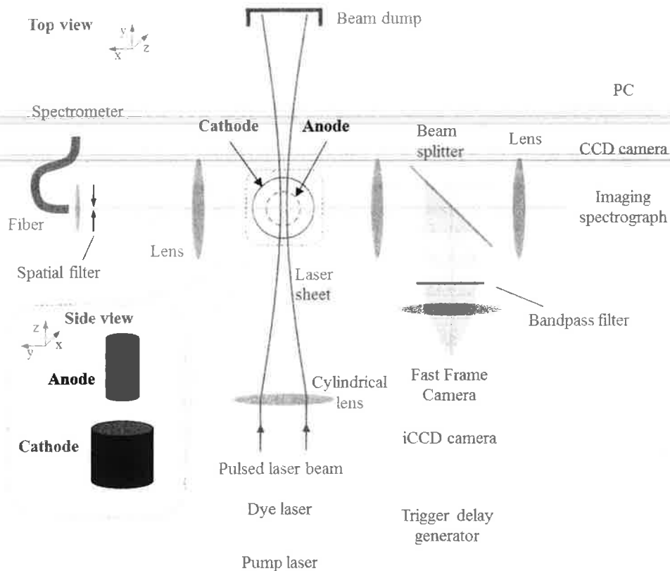
Fig.1 Schematic of the experimental setup of carbon arc for synthesis of carbon nanotubes.
