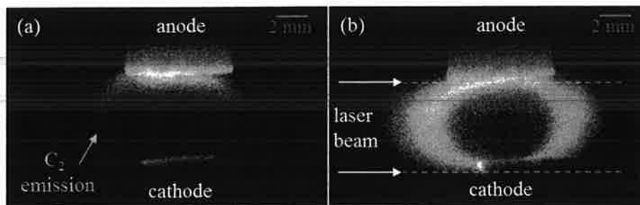
Fig. 5. Emission pattern of C_2 with laser (a) off and (b) on (PLIF). Graphite electrodes, configuration C9-A6, 50 A, exposure time 20 ns.
