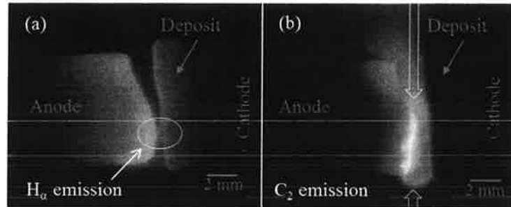
Fig. 6. Simultaneous frames of the arc H_{\alpha} (a) and C_2 (b) emission in high ablation mode (graphite electrodes, configuration C9-A6, 65 A, exposure time 2 \mu s). Intensity and colors were artificially adjusted to enhance visualization of the emission patterns.
