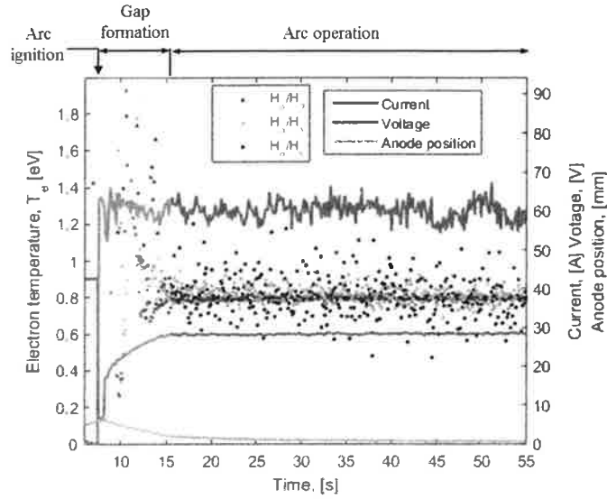
Fig. 8. Time evolution of the arc core plasma electron temperature during an arc run. The temperature (dotted plot) was calculated from ratios of H_{\alpha}/H_{\beta} (red), H_{\alpha}/H_{\gamma} (green) and H_{\alpha}/H_{\delta} (blue). Solid lines are waveforms of discharge current (blue), voltage (dark red) and axial position of the anode (yellow).
