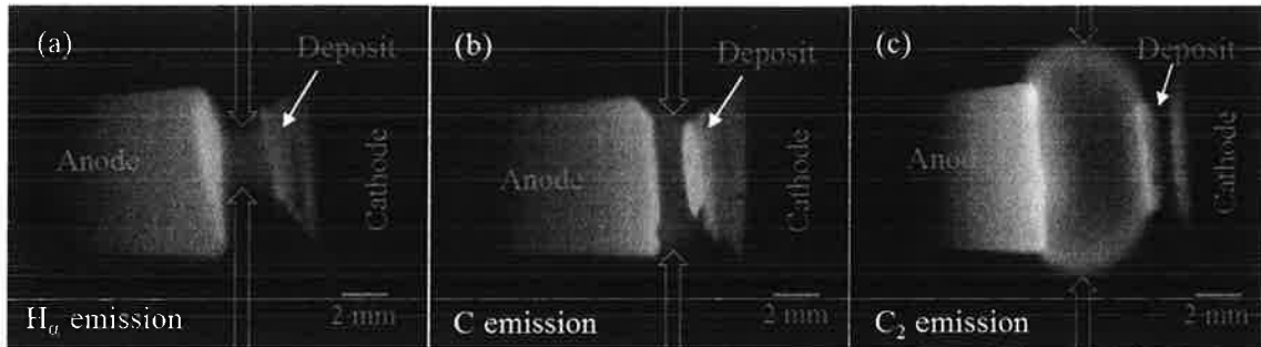
Fig. 3. Spectral images of H_\alpha (a), C I (b), and C_2 (c) obtained by FFI with the arc operated in the low ablation mode (graphite electrodes, configuration C9-A6, 50 A). Intensity and colors were artificially adjusted to enhance visualization of the emission patterns.
