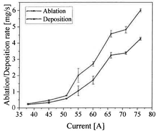
Fig. 2. Ablation and deposition rates as a function of the discharge current. Electrode configuration C9-A6, helium gas at 67 kPa.
