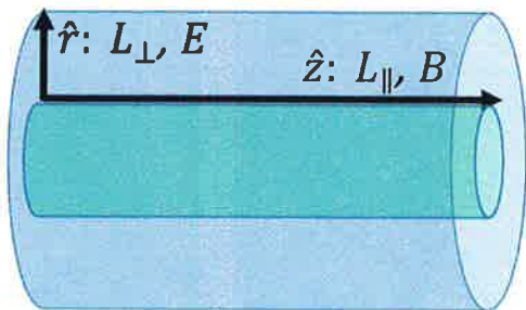
FIG. 1. Relevant length scales and fields in simplified PMF model. Ions must remain confined in an annular region of width L_{\perp} between the green and blue cylinders while they exit axially. In this paper, we focus on the transport of the minority heavy ions, which are more likely to be long-lived, radioactive isotopes. The E field points radially, perpendicular to the axial B field.
