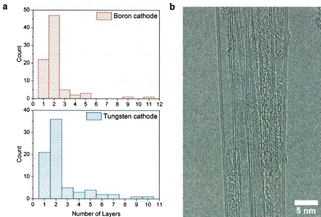
Figure 1: (a) BNNTs synthesized with boron and tungsten cathodes show similar results. The tubes were primarily single and double walled. (b) A bundle of double walled BNNTs.
