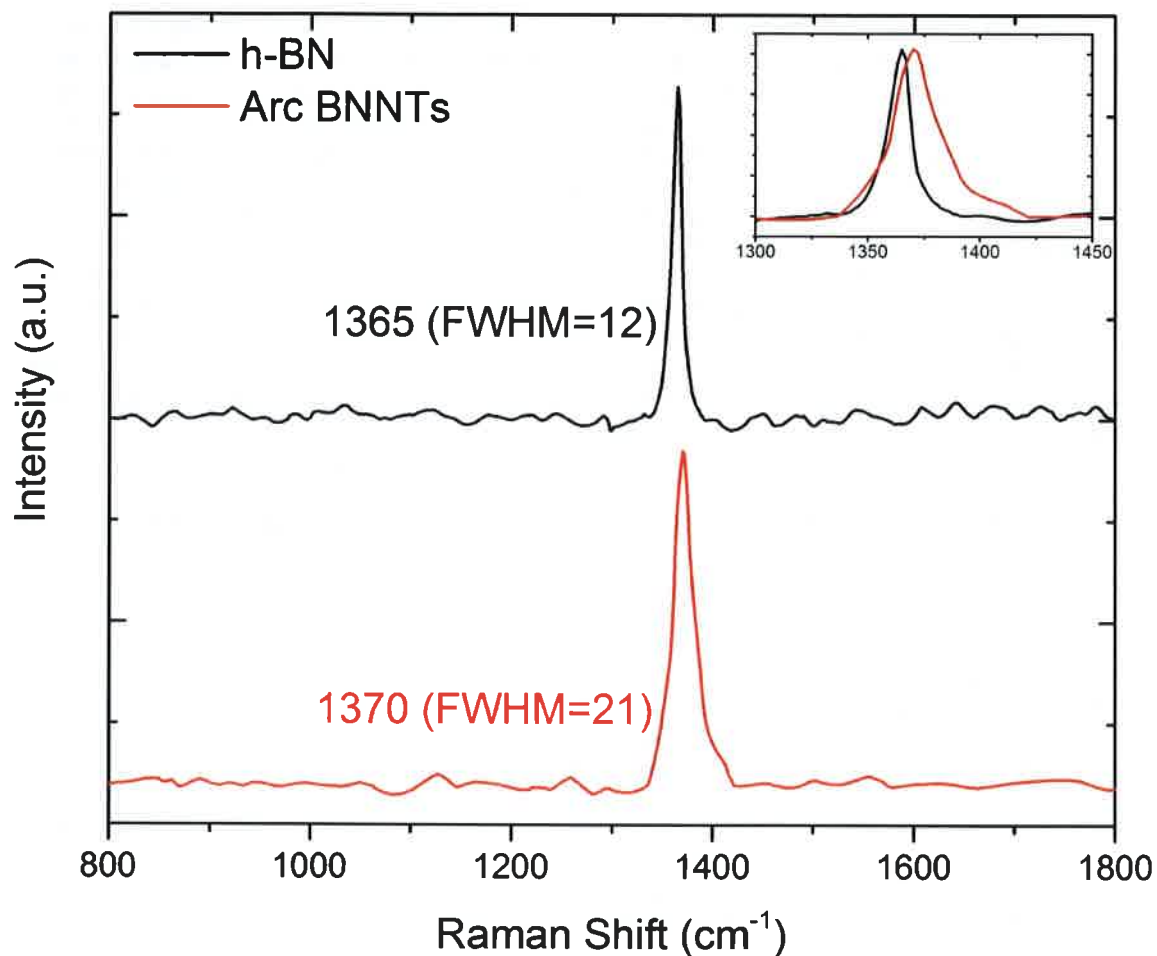
Figure 5: Raman spectra of bulk hexagonal boron nitride powder (black) and the arc synthesized BNNTs (red). Only the E_{2g} mode of hexagonal boron nitride was observed, and the blue shift observed in the synthesized BNNTs is characteristic of few-layer boron nitride.
