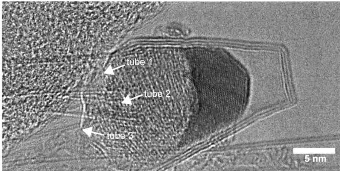
Figure 2: Three BNNTs grown out of an unreacted anode nanoparticle. The particle is also wrapped by boron nitride layers.
