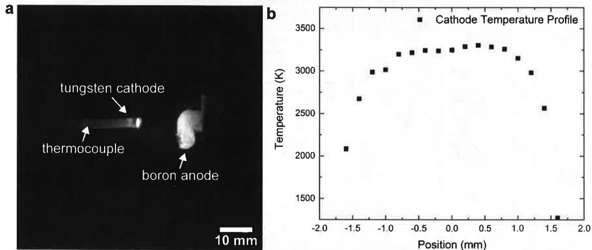
Figure 3: (a) IR image of the electrodes during the arc discharge. (b) Temperature profile of the plasma facing tungsten cathode tip. A position of zero corresponds to the center along the width of the electrode (3.2 mm dia.), with other relative positions toward the electrode edge indicated.
