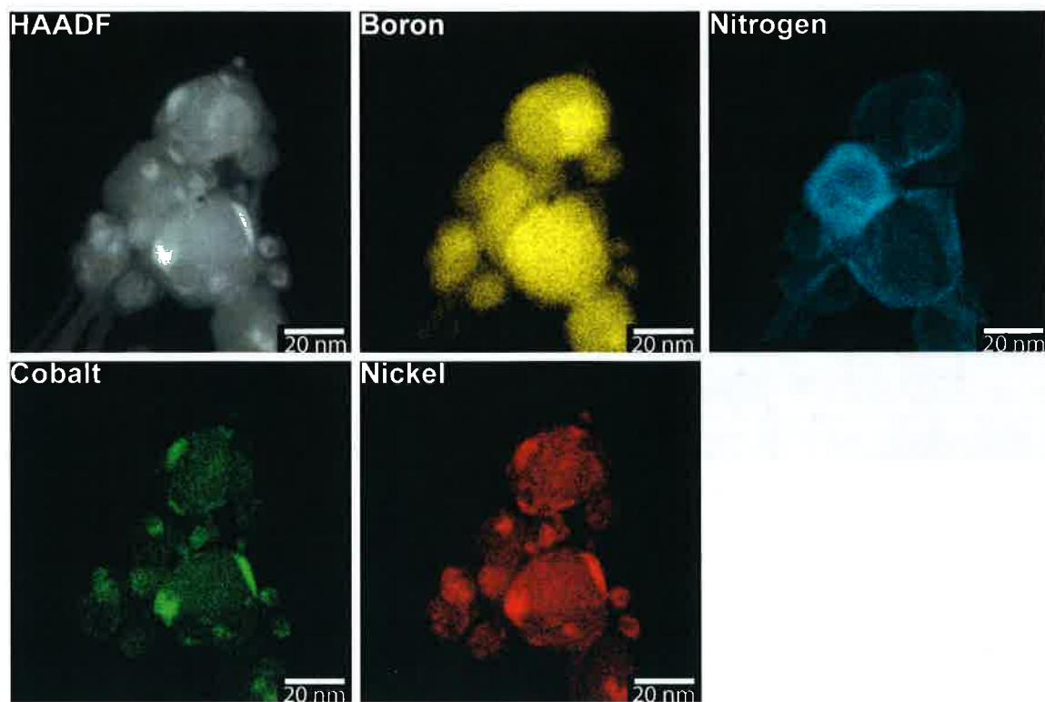
Figure 4: EDS elemental mapping results. The particles contain boron, cobalt, and nickel, characteristic of the starting anode material used in the arc synthesis. Boron and nitrogen mapping results show that the tube bundles on the lower left are boron nitride and the nanoparticles are wrapped by boron nitride.
