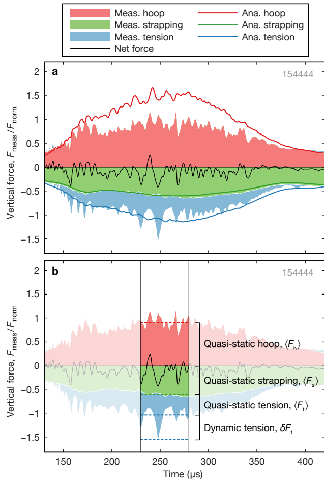
Figure 4. (a) Comparison of experimentally measured (solid patches) and analytically predicted (colored lines) forces for a sample flux rope discharge. The net measured force is shown in black. The forces are normalized to F_{\text{norm}} \equiv \mu_0 I_T^2 / 4\pi x_f , where I_T is the toroidal plasma current and 2x_f is the footpoint separation distance. A force-free equilibrium is measured, which confirms that these experiments are low- \beta . The measured hoop force is weaker than the analytical prediction, while the tension and strapping forces are comparable. (b) The various force terms are condensed to scalar values by averaging over the time when the plasma current is within 5% of its maximum. Regarding the tension force, the quasi-static contribution, \langle F_t \rangle , is the average of the low-pass-filtered tension force, while the dynamic contribution, \delta F_t , is the maximum transient in excess of \langle F_t \rangle . In this example, \delta F_t is larger in magnitude than \langle F_t \rangle , indicating that the dynamic tension force can be significant.
