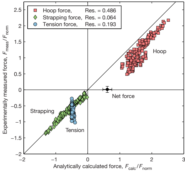
Figure 5. Comparison of measured and predicted quasi-static flux rope forces. Again, the forces are normalized to F_{\text{norm}} \equiv \mu_0 I_T^2 / 4\pi x_f . The measured hoop force is weaker than predicted, the strapping force is well-predicted, and the tension force can exceed predicted values by as much as a factor of two. When the various force terms are summed, a force-free equilibrium (zero net force) is measured but not predicted. This figure reprinted with permission from Ref. 4.
