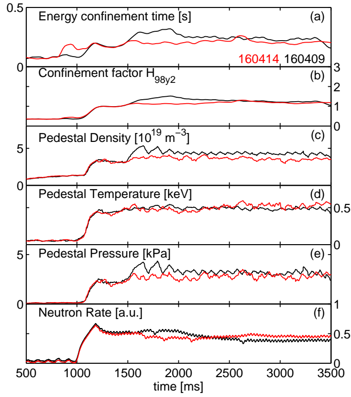
Figure 11. Evolution of selected parameters representative of the discharge performance and pedestal characteristics, for discharges 160414 (LGI) and 160409 (reference), also shown in Fig. 6.
