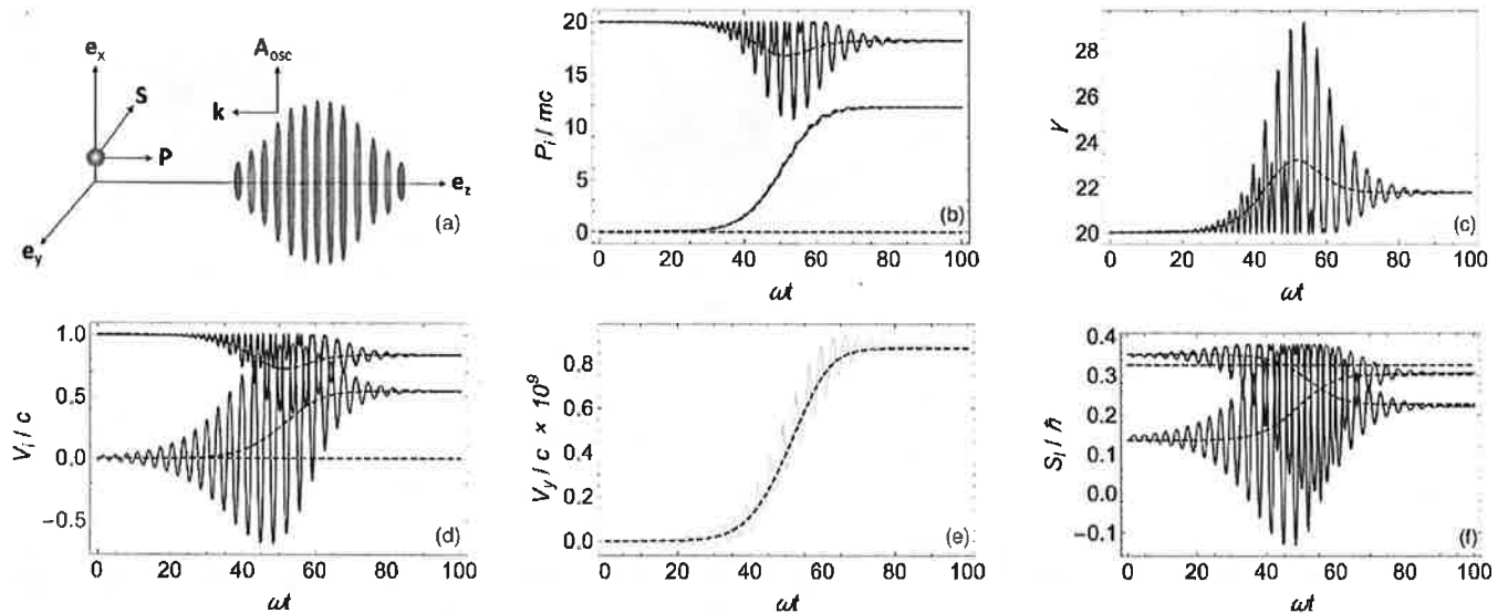
FIG. 1: Motion of a single Dirac electron under the action of a relativistically intense laser pulse (numerical simulation): black dashed – ponderomotive model described by the Lagrangian (75); colored – XBMT model described by the Lagrangian (91). (a) Schematic of the interaction; yellow and red is the laser field, blue is the particle; arrows denote the direction of the laser wave vector \mathbf{k} , the oscillating vector potential \mathbf{A}_{\text{osc}} , the particle canonical momentum \mathbf{P} , and the particle spin \mathbf{S} . The unit vectors along the reference axes are denoted by \mathbf{e}_i . Figures (b)-(f) show the components of the particle canonical momentum \mathbf{P} , Lorentz factor \gamma , velocity \mathbf{V} , and spin \mathbf{S} . The red, green, and blue lines correspond to projections on the x , y , and z axes, respectively. We consider an electron initially traveling along the z -axis and colliding with a counter-propagating laser pulse. The initial position of the particle is \mathbf{X}_0 = (\ell/2)\mathbf{e}_x , the initial momentum is \mathbf{P}_0/(mc) = 20\mathbf{e}_z , and the normalized initial spin vector is \mathbf{S}_0/\hbar = 0.14\mathbf{e}_x + 0.33\mathbf{e}_y + 0.35\mathbf{e}_z . The envelope of the vector potential of the laser pulse is q\mathbf{A}_{\text{osc}}/(mc^2) = 30 \text{sech}[(z - 5\ell + ct)/\ell] \exp[-(x^2 + y^2)/\ell^2] \mathbf{e}_x , where \ell = 20|\mathbf{k}|^{-1} . These parameters correspond to a maximum intensity I_{\text{max}} \simeq 1.23 \times 10^{21} \text{ W/cm}^2 for a 1 \mu\text{m} laser.
