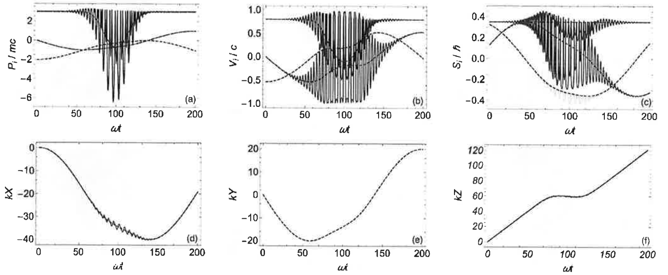
FIG. 2: Motion of a Dirac electron under the action of an external background field and a relativistically intense laser pulse (numerical simulation): black dashed – ponderomotive model described by the Lagrangian (75); colored – XBMT model described by the Lagrangian (91). Figures (a)-(c) show the components of the particle canonical momentum \mathbf{P} , velocity \mathbf{V} , and spin \mathbf{S} . The red, green, and blue lines correspond to projections on the x , y , and z axes, respectively. We consider an electron initially traveling along the z -axis and colliding with a counter-propagating laser pulse. Figures (d)-(f) show the components of the particle position \mathbf{X} . The initial position of the particle is \mathbf{X}_0 = \mathbf{0} , the initial momentum is \mathbf{P}_0/(mc) = (-2\mathbf{e}_y + 3\mathbf{e}_z) , and the normalized initial spin vector is \mathbf{S}_0/\hbar = 0.14\mathbf{e}_x + 0.33\mathbf{e}_y + 0.35\mathbf{e}_z . A background magnetic field is added such that q\mathbf{A}_{bg}/(mc^2) = 0.1(-y\mathbf{e}_x + x\mathbf{e}_y)/2 , which corresponds to a static homogeneous magnetic field B_{bg} \simeq 10.7 MG aligned towards the z -axis. The envelope of the vector potential of the laser pulse is assumed to have the form q\mathbf{A}_{osc}/(mc^2) = 10 \operatorname{sech}[(z - 8\ell + ct)/\ell] \mathbf{e}_x , where \ell = 20|\mathbf{k}|^{-1} . These parameters correspond to a maximum laser intensity I_{\max} \simeq 1.37 \times 10^{20} W/cm 2 for a 1 \mu m laser.
