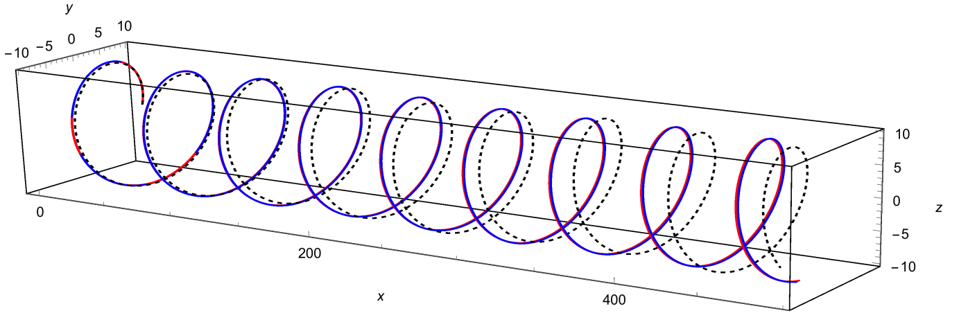
FIG. 1: Comparison between ray trajectories predicted by the canonical Lagrangian (76) and the non-canonical Lagrangian (81). The red line represents \mathbf{X}(t) - \mathbf{A}(\mathbf{P}(t)) , where \mathbf{X}(t) and \mathbf{P}(t) are found by numerical integration of Eqs. (78) and (79). The blue line shows \mathbf{x}(t) , as found by numerical integration of Eqs. (90) and (91). The black dashed line plots the “spinless” ray trajectory governed by the lowest-order GO ray Lagrangian L_0 given by Eq. (93). The refraction index is chosen to be n(\mathbf{x}) = 1 + \exp[-(y^2 + z^2)/\ell^2] , the characteristic width is \ell = 10 , and \mathbf{A} is chosen in the form (50). The length unit is a \doteq \sqrt{2}/p_0 . The initial location is \mathbf{x}_0 = (0, 10, 0) , and the initial momentum is \mathbf{p}_0 = (1, 0, 1)/a , so \epsilon \sim 1/(p_0\ell) \sim 0.07 . It is seen that the canonical Lagrangian and the noncanonical Lagrangian predict results that, for the specified parameters, are essentially indistinguishable from each other yet differ noticeably from those yielded by L_0 .
