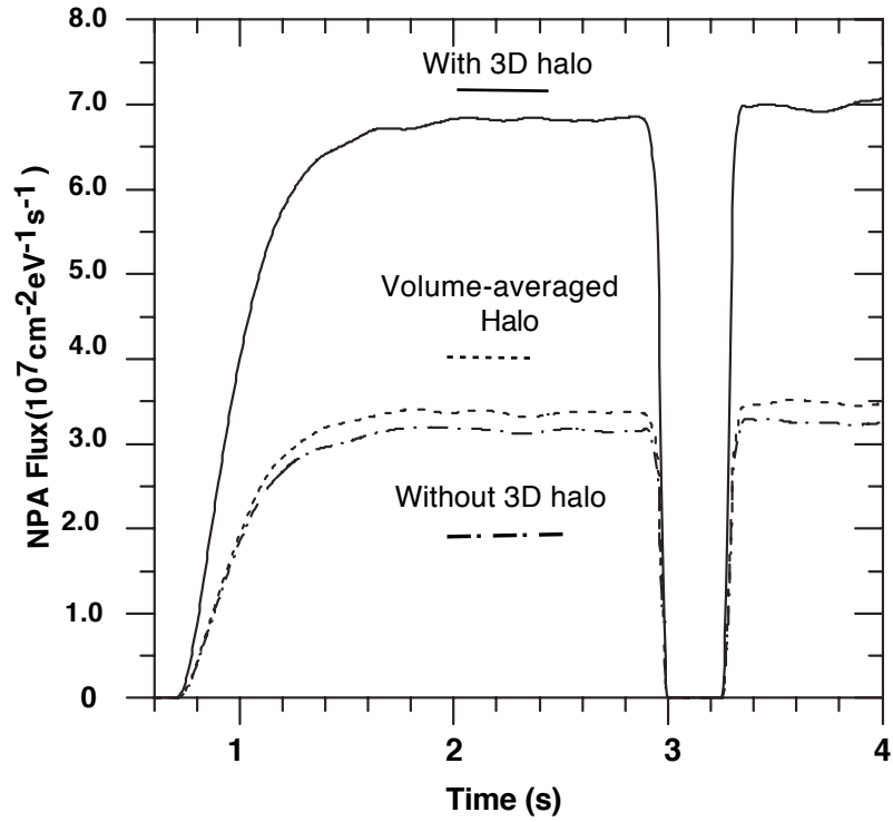
Fig. 14. Comparison of the charge exchange neutral flux time evolution at E = 85 \text{ keV} for the ssNPA sightline with and without 3D halo neutrals. Also shown is the effect of volume-averaging the 3D halos.
