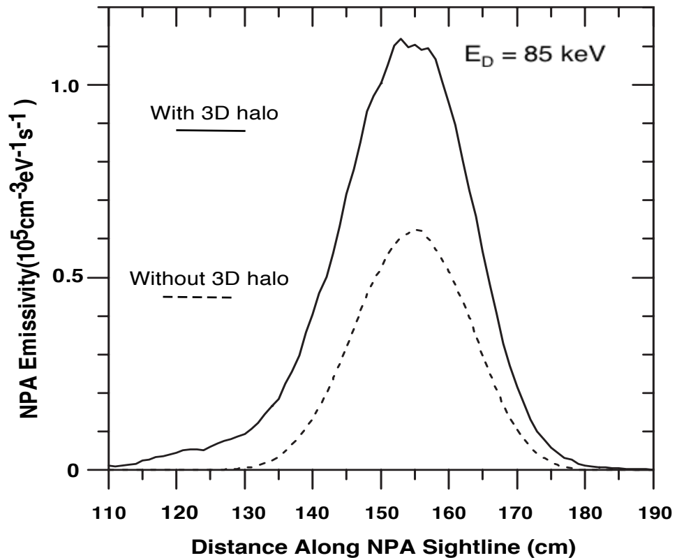
Fig. 9. Comparison of the charge exchange neutral emissivity for the E1B NPA sightline with and without 3D halo neutrals.
