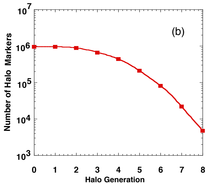
Fig. 2. Schematic of the 3D halo neutral generation process (a) and a typical example of 3D halo generation evolution from the NUBEAM code (b).
