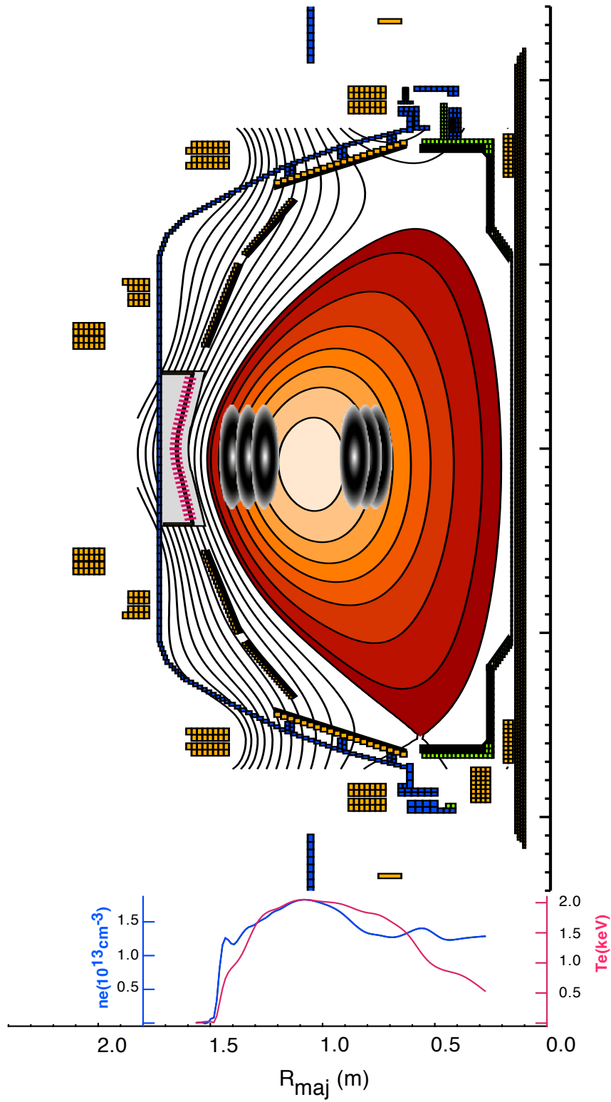
Fig. 4. The NPA flux is localized by the intersection of the diagnostic sightlines with NBI footprints as illustrated by shaded black ovals. The inner triad corresponds to NBI#1 and the outer triad to NBI#2.
