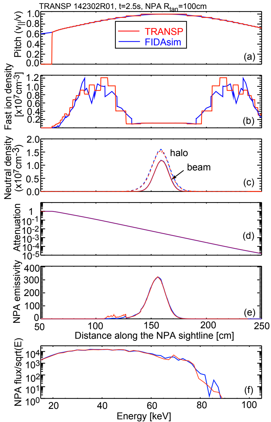
Fig. 21. Benchmarking of the NPA simulator in the TRANSP and FIDASim codes with a projected NSTX-U discharge. Both TRANSP and FIDASim use the plasma profiles from TRANSP Run ID 142302R01 at t = 2.5s . (a) Pitch angle that can reach the NPA detector (b) fast ion density at the pitch angle that can reach the NPA detector, (c) beam and halo neutral densities, (d) attenuation factor for 60 keV neutrals, (e) emissivity along the NPA sightline and (f) NPA energy spectrum for a sightline with both beam and halo neutrals.
