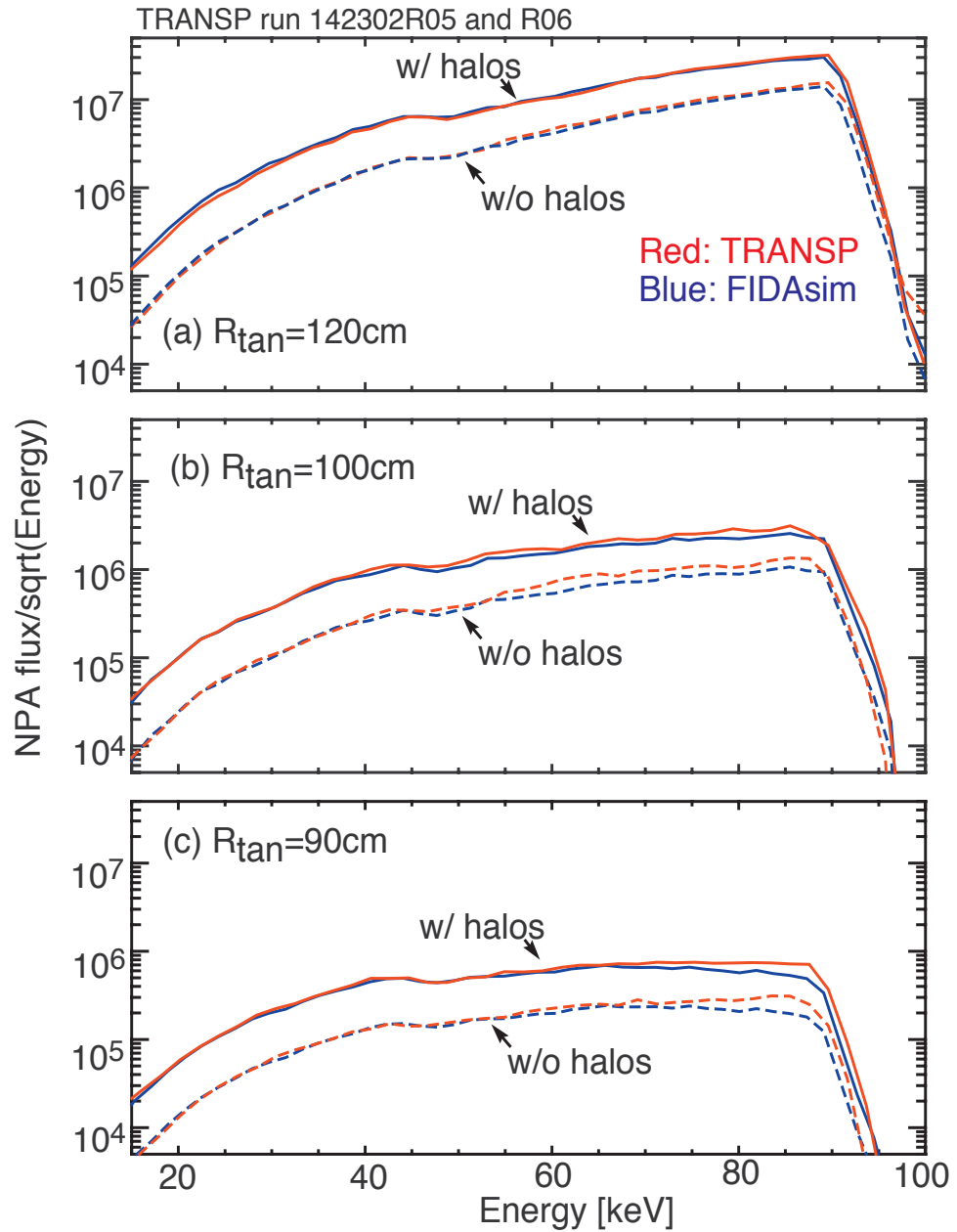
Fig. 19. Comparison of NPA energy spectrum at t = 2.5 s with and without halo neutrals for the NPA sightlines captioned in (a), (b), and (c). The TRANSP simulation results are shown in red, and the FIDASIM simulation results are plotted in blue. The TRANSP and FIDASIM simulation results overlap with each other.
