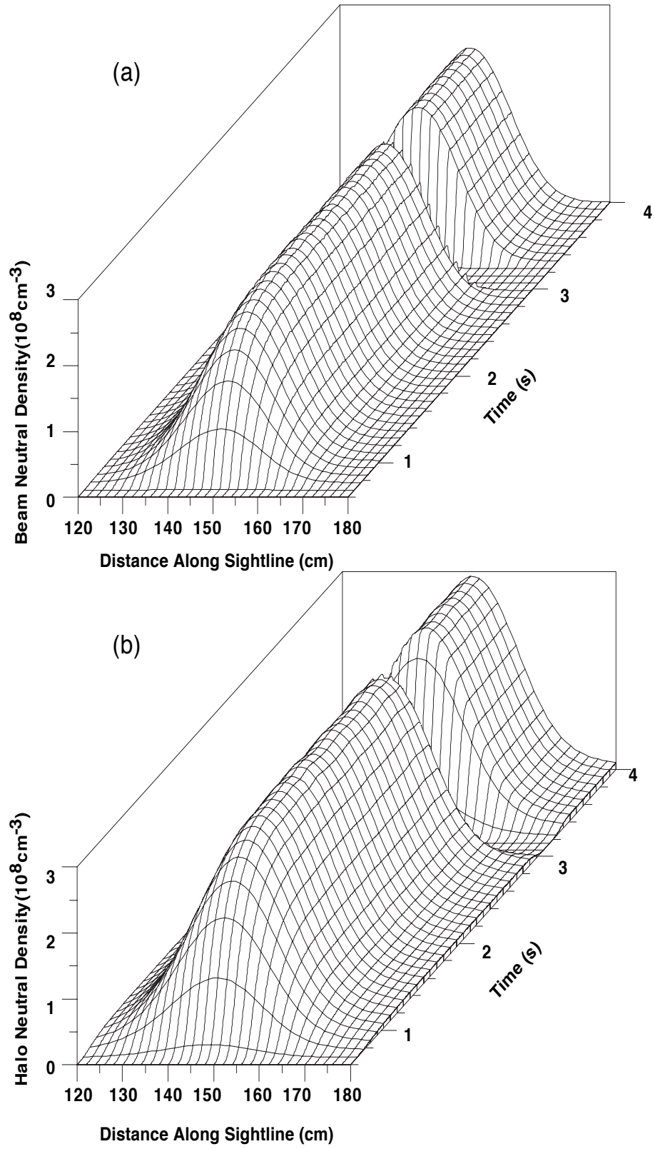
Fig. 5. Injected beam neutral density (a) and halo neutral density (b) as a function of distance along the EIB NPA sightline depicted in Fig. 4.
