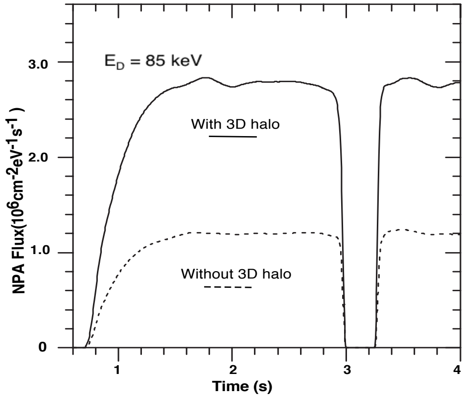
Fig. 8. Comparison of the charge exchange neutral flux time evolution at for the E1B NPA sightline with and without 3D halo neutrals.
