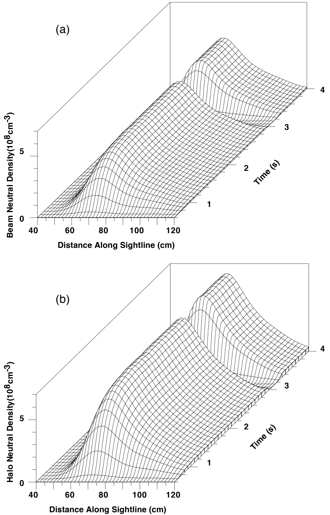
Fig. 11. Injected beam neutral density (a) and halo neutral density (b) as a function of distance along the ssNPA sightline depicted in Fig. 4.
