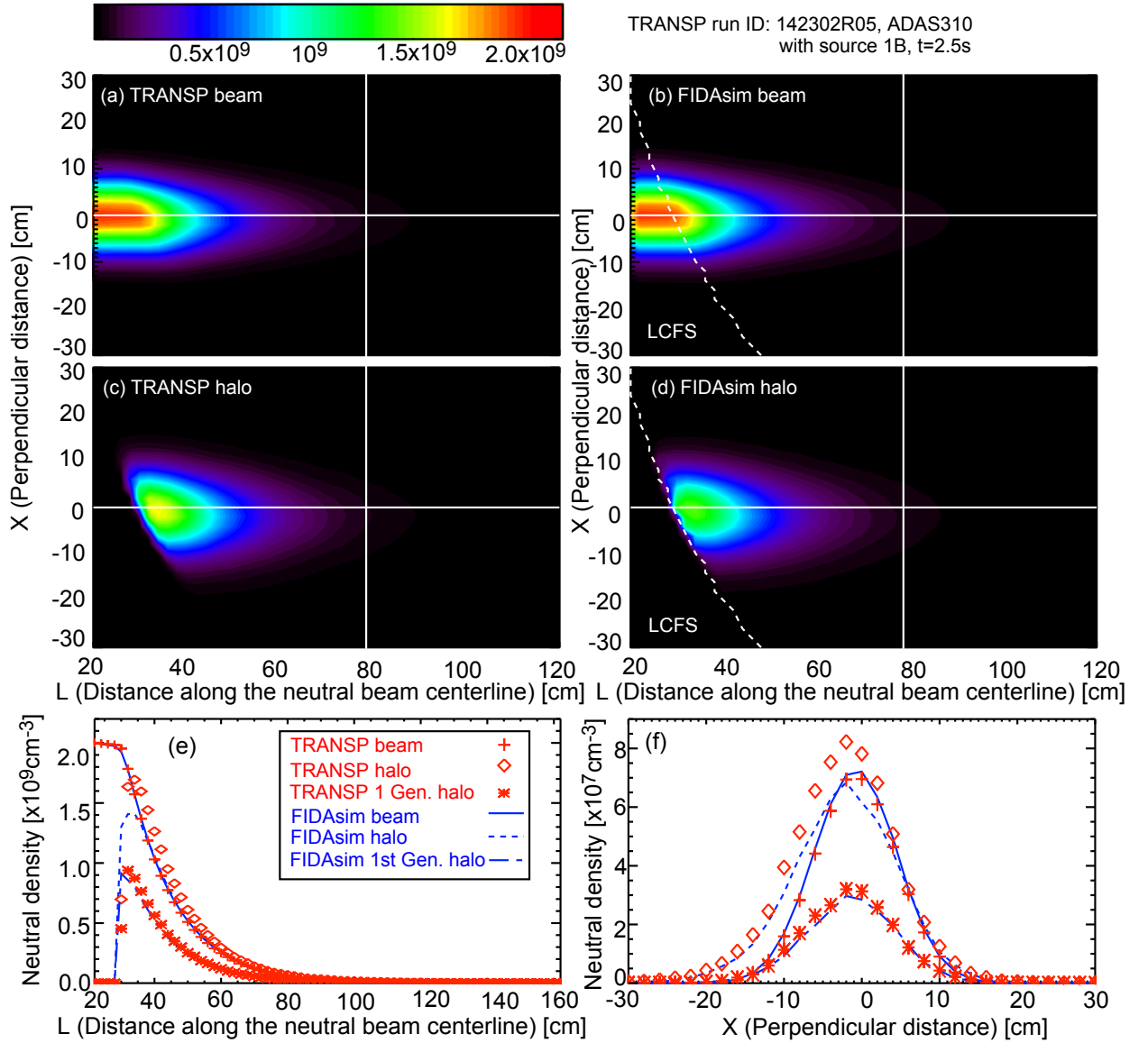
Fig. 23. Comparison of TRANSP and FIDASim calculated beam and halo neutral densities for a NSTX-U projected discharge when TRANSP and FIDASim use their own standard cross section tables. TRANSP uses ADAS310, while FIDASim mainly uses ADAS and Janev 2004 report. (a) TRANSP and (b) FIDASim simulated beam neutral density on the midplane. (c) TRANSP and (d) FIDASim simulated halo neutral density on the midplane. (e) Comparison of beam and halo neutral densities along the white overlaid horizontal lines from the contour plots in the panels (a)-(d). (f) Comparison of beam and halo neutral densities along the white overlaid vertical lines from the contour plots in panels (a)-(d). The same color bar is used for all contour plots in the panels (a)-(d).
