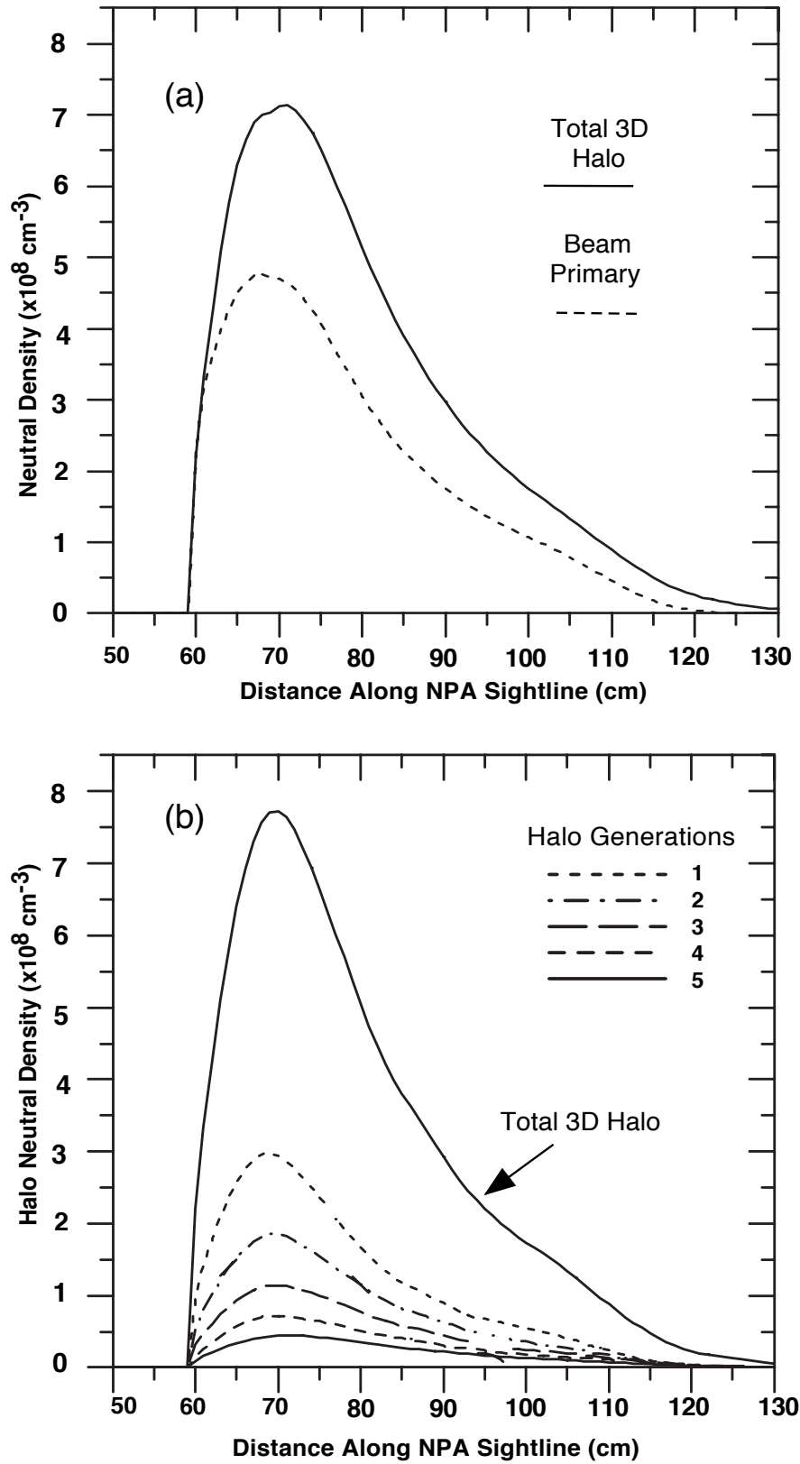
Fig. 12. Comparison of beam primary and total halo neutral densities (a) and the composition of the halo neutral density over multiple generations (b) as viewed along the ssNPA sightline.
