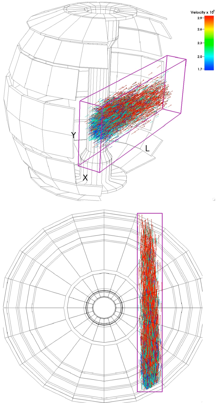
Fig. 1. Illustration of “beam-in-box” model for the TRANSP 3D halo neutral code. Note only beam primary neutrals are shown.
