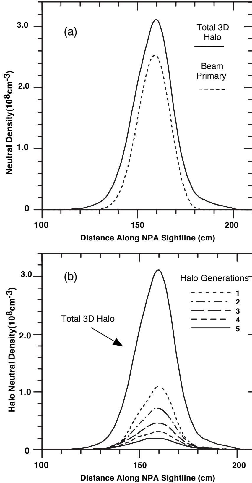
Fig. 6. Comparison of beam primary and total halo neutral densities (a) and the composition of the halo neutral density over multiple generations (b) as viewed along the E11B NPA sightline.
