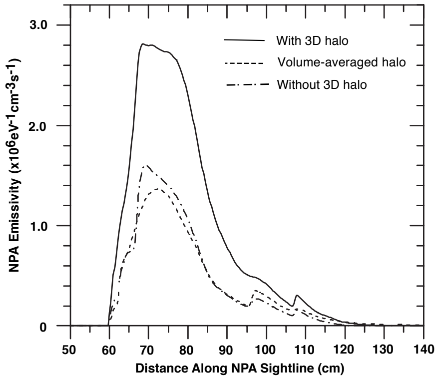
Fig. 15. Comparison of the charge exchange neutral emissivity at E = 85 \text{ keV} for the ssNPA sightline with and without 3D halo neutrals. Also shown is the effect of volume-averaging the 3D halos.
