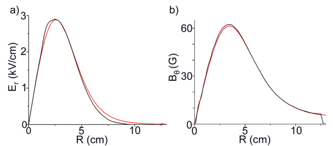
FIG. 4. Comparison of (a) the E_r fields and (b) the B_\theta fields from the analytic model of Ref. 27 and LSP particle-in-cell simulation for the case of n_p = n_b/5 with electron emitters on the chamber walls. These are radial slices taken at the center of the beam. Red represents the analytic model and black represents the LSP simulation. There is close agreement.
