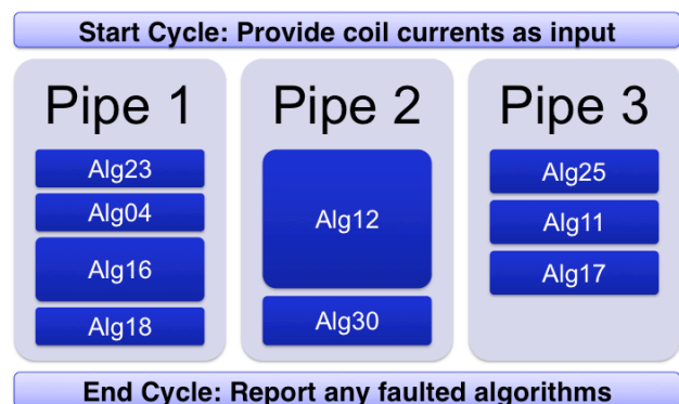
Fig. 3. Algorithm Pipelining Scheme
