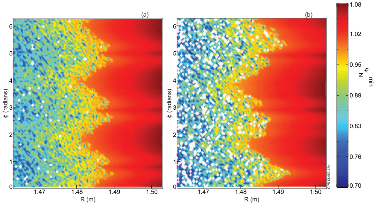
Figure 13. MAST A laminar plot generated by the ERGOS code showing the minimum normalised flux experienced by each field-line traced from each given poloidal position in one toroidal plane. The field-lines are followed for 200 toroidal turns or until they reach the divertor target. The deformation of the ‘boundary’ in MAST when an n = 3 (a) even parity and (b) odd parity RMP is applied predicted by ERGOS is \pm 5 - 6 mm, which is significantly less than the displacement measured experimentally [26], where a displacement of \pm 2.5 cm is observed when the RMPs are switched on.
