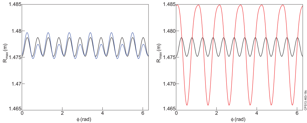
Figure 18. MAST The plasma boundary predicted by VMEC for a MAST connected double null plasma when an n=6 RMP is applied compared to the case with no RMP but with toroidal field ripple when the RMP has (left) even parity configuration and (right) an odd parity configuration.
