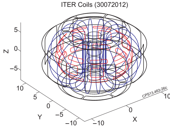
Figure 26. The coil set used in ITER simulations, with the in-vessel control coils marked in red.
