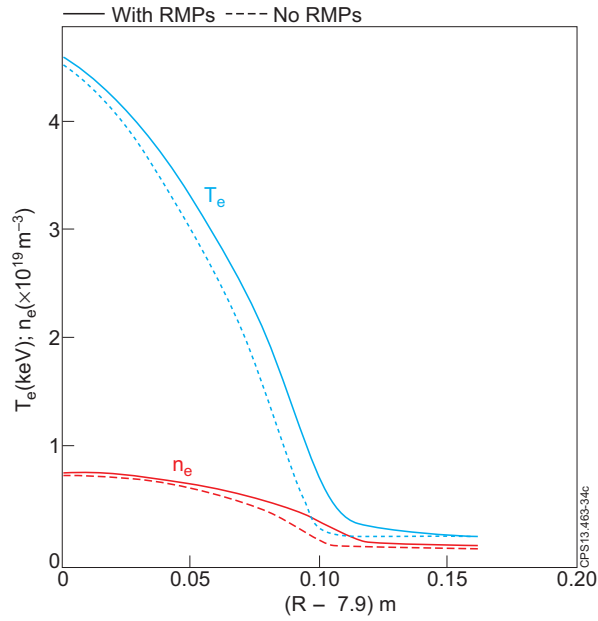
Figure 33. ITER The electron density and temperature as a function of the minor radius as predicted by a non-linear JOEKE simulation when 55kAt is applied in n = 3 configuration.
