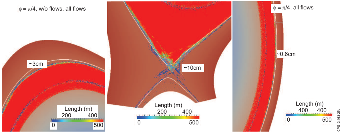
Figure 25. JET Poincare plots showing the (left) top, (middle) lower X-point region and (right) midplane of JET discharge 77329 modelled using JOREK when realistic diamagnetic and toroidal flows are included.
