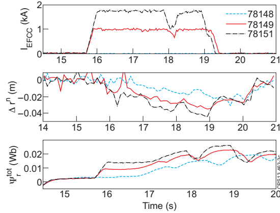
Figure 3. JET The RMP-induced displacement measured by the Thomson scattering diagnostic as a function of time (centre) compared to the current in the ex-vessel coils in JET (top) and change in the magnetic flux (bottom).
