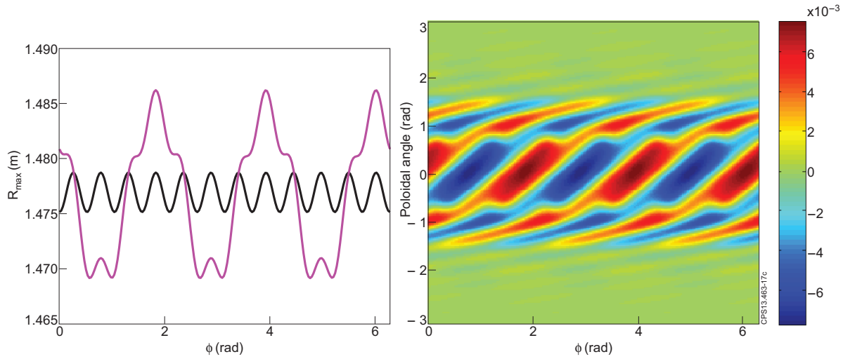
Figure 16. DIII-D The plasma boundary displacement as a function of toroidal and poloidal angles as predicted by the STELLOPT code for a DIII-D plasma with an n = 3 RMP applied.
