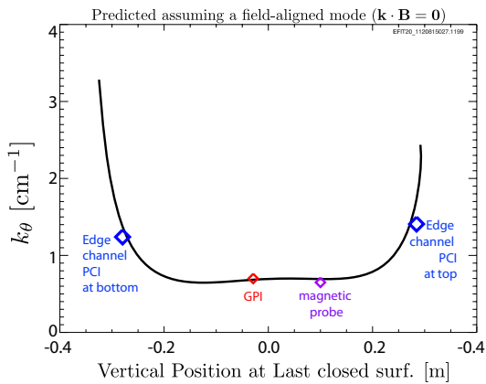
FIG. 6: (color online) Predictions of the poloidal wavenumber as a function of the vertical position assuming that the instability is field-aligned. Overlaid are the vertical positions of the different diagnostics used in this work to show agreement in wave numbers.
