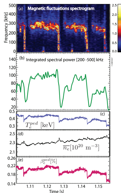
FIG. 4: (color online) (a) Magnetic fluctuations spectrogram displaying the inter-ELM fluctuations sustained for 10 - 20 ms. (b) Integrated spectral amplitude obtained from integrating the above spectrogram between 200 and 500 kHz. (c) Edge temperature evolution measured using the ECE. (d) Line-averaged density evolution. (e) Estimate of the pedestal electron \beta evolution.
