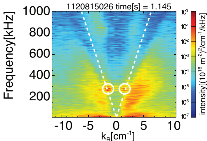
FIG. 1: (color online) (a) Wavenumber-frequency spectrum of observed PCI fluctuations displaying a mode coherent in both frequency and radial wavenumber. From this spectrum, we determine a phase velocity of \pm 12 km/s as labelled with the oblique dotted lines.
