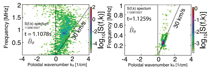
FIG. 5: (color online) Frequency-wavenumber spectra of the magnetic fluctuations for two distinct time slices; [Left]: before the onset of instability and [right]: saturated regime. In both panels, an oblique lines is displayed to show the corresponding phase velocity of 30 km/s.
