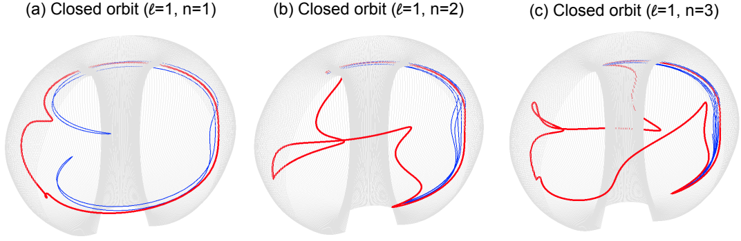
FIG. 4: 3D particle trajectories of the closed orbit with \vec{E} \times \vec{B} (red) compared to the original banana orbit (blue) in NSTX. The closed orbit of the \ell -class particle toroidally circulates \ell cycles for n bounces as shown for (a) (\ell, n)=(1, 1) , (b) (1, 2) , and (c) (1, 3) .
