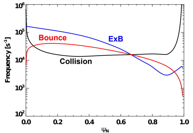
FIG. 11: Frequency profiles of the ion collision, the electric precession, and the ion bounce motion for the NSTX 124439. It is indicated that the plasma is in \nu - \sqrt{\nu} regime at the core and in 1/\nu regime at the edge. Bounce-harmonic resonances take dominant effects in the whole region due to fast toroidal rotation.
