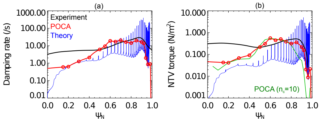
FIG. 13: Comparison of (a) rotational damping rate and (b) NTV torque profile between measurement (black), POCA (red) and theory (blue) for NSTX discharge 124439. Total NTV torque is measured at 3.5 Nm, and agrees well with 2.7 Nm from POCA in spite of discrepancies in the profile. NTV profile by POCA with n_c = 10 is drawn for comparison (green), showing a poor agreement at the edge due to less accurate fitting of \delta B .
