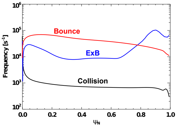
FIG. 8: Frequency profiles of ion collision, electric precession, and ion bounce motion for the DIII-D 145117. It is indicated that the plasma is in the \nu_- \sqrt{\nu} regime, however, bounce-harmonic resonance can be important at the edge.
