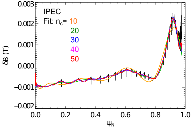
FIG. 7: Sensitivity of Chebyshev fitting to the degree of polynomials. \delta B profiles for NSTX 124439 in Fig. 6(a) are taken.
