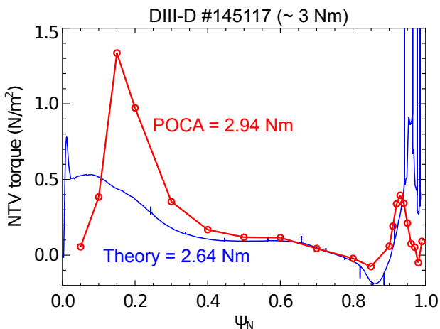
FIG. 9: NTV profiles for DIII-D discharge 145117 by POCA (red) and the combined theory (blue). Both calculations provide a reasonable prediction in total NTV torque (2.94 Nm by POCA, 2.64 Nm by theory), which is estimated at \sim 3 Nm in the experiment.
