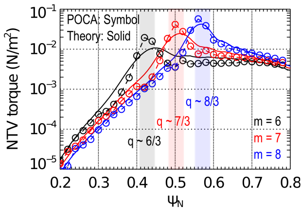
FIG. 2: NTV torque profiles by ( m = 6, 7, 8, n = 3 ) modes. Strong NTV peaks appear at the resonant flux surfaces where q = 6/3, 7/3, and 8/3 for each poloidal mode number.
