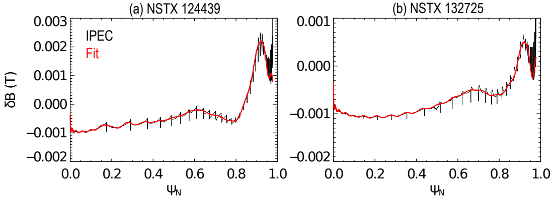
FIG. 6: Comparison of non-axisymmetric magnetic field profiles between IPEC and fitting with Chebyshev polynomials for NSTX discharge (a) 124439 and (b) 132725. Profiles are taken at (\theta, \varphi) = (0, 0) with n_c = 20 . Fittings efficiently smooth the nonphysical peaks but reflect overall features of the original IPEC calculation well.
