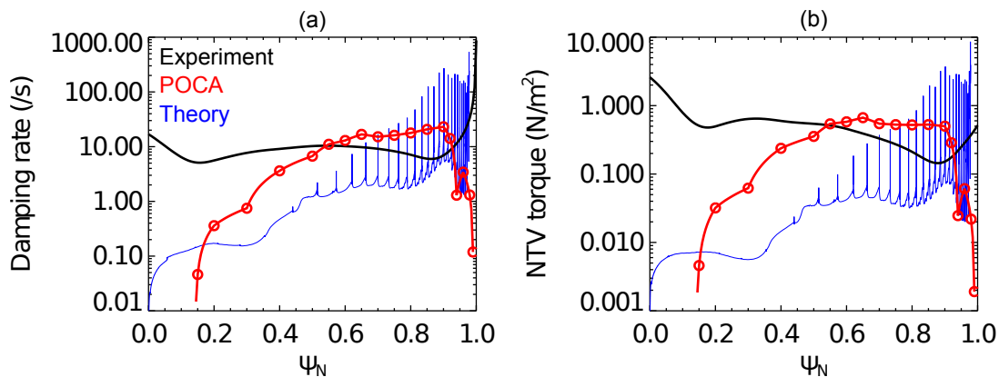
FIG. 14: Comparison of (a) the rotational damping rate and (b) the NTV torque profile among measurement (black), POCA (red), and theory (blue) for NSTX discharge 132729.
