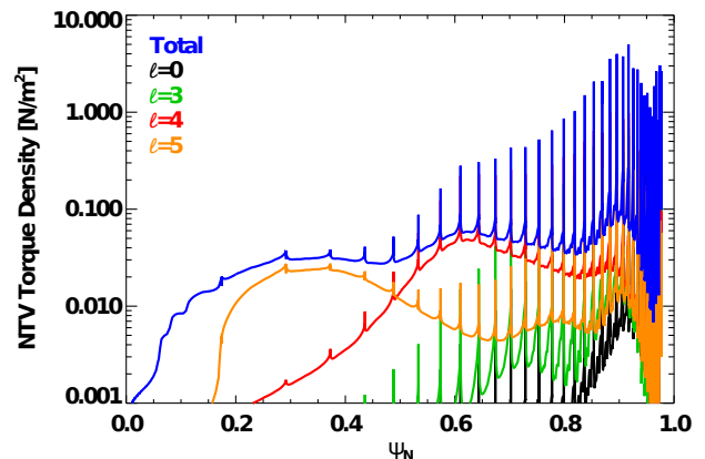
FIG. 12: NTV profiles calculated by the combined formula for dominant \ell -classes. Bounce-harmonic resonances are found to take dominant effects in the overall region due to fast toroidal rotation, and \ell = 0 particles take local effects at the edge.
