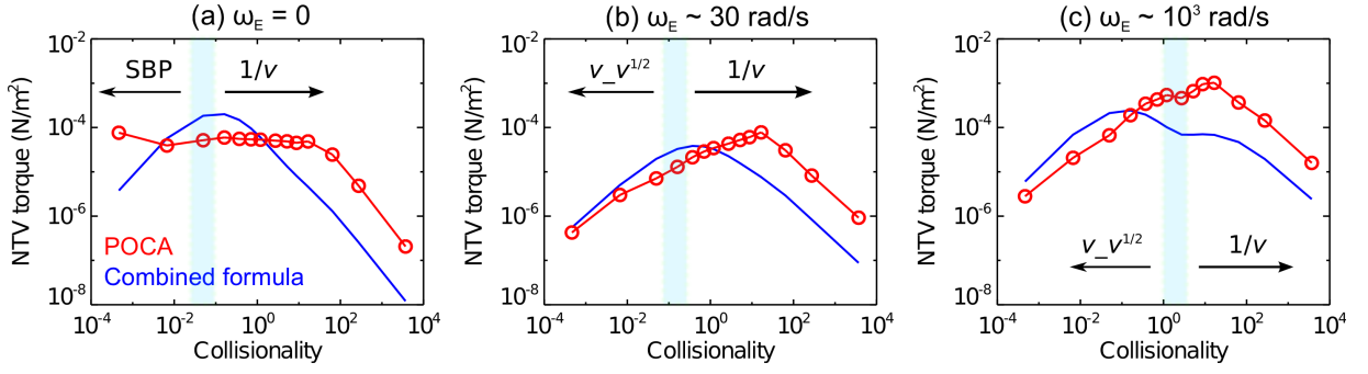
FIG. 3: Comparison of NTV between POCA (red-symbol) and combined formula (blue-solid) as a function of collisionality with fixed \vec{E} \times \vec{B} frequency at (a) \omega_E = 0 , (b) \omega_E \sim 30 rad/s, and (c) \omega_E \sim 10^3 rad/s. Shaded is the theoretically estimated boundary (a) for SBP and 1/\nu regime, and (b)(c) for \nu-\sqrt{\nu} and 1/\nu regime.
