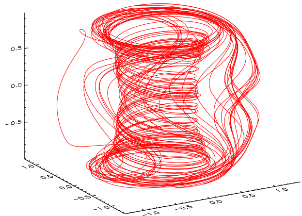
FIG. 1: 3D trajectory of a single guiding-center orbit motion in an axisymmetric NSTX plasma, calculated by POCA. Collisions were neglected here.
