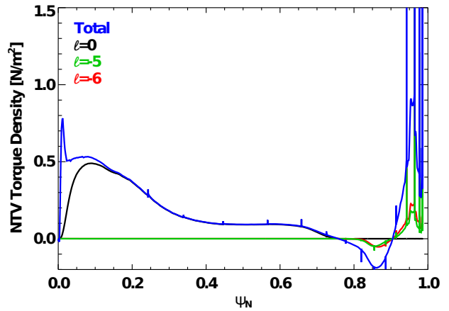
FIG. 10: NTV profiles calculated by the combined formula for dominant \ell -classes. Bounce-harmonic resonances are found to be important only in the pedestal due to slow toroidal rotation in the discharge.
