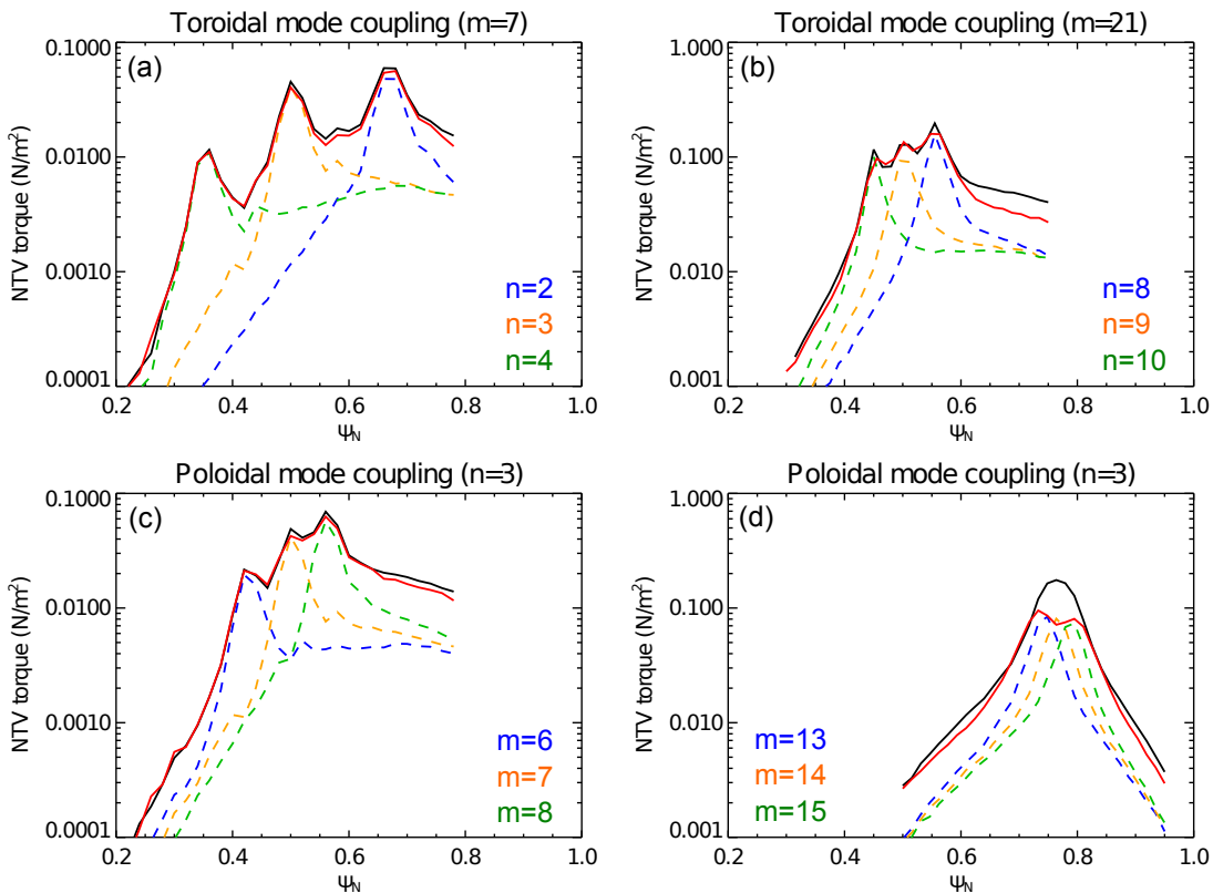
FIG. 5: Comparisons of NTV profiles between three-mode (red) and linear sum of single-mode (black) perturbations. Three-modes are considered with the fixed poloidal mode for (a) and (b), and the fixed toroidal mode for (c) and (d). Broken curves indicate the NTV profiles by single-mode perturbation, and black solid curve does their sum.
