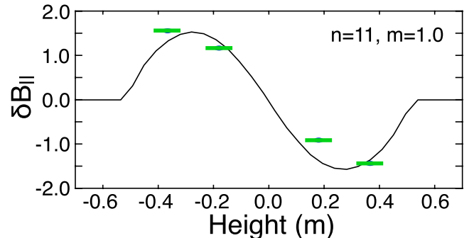
FIG. 9. Comparison of simulated (black line) and experimental (green bars) magnetic fluctuations at the wall for the mode shown in Fig. 8(b).
