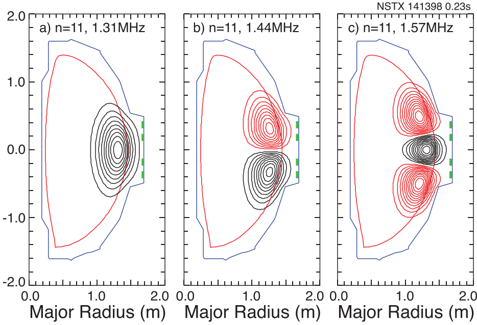
FIG. 8. Approximate eigenmodes for the first three poloidal eigen-states with n = 11 . (a) The lowest order n = 11 poloidal eigen-state, (b) the second order n = 11 poloidal eigen-state, and (c) the third order n = 11 poloidal eigen-state.
