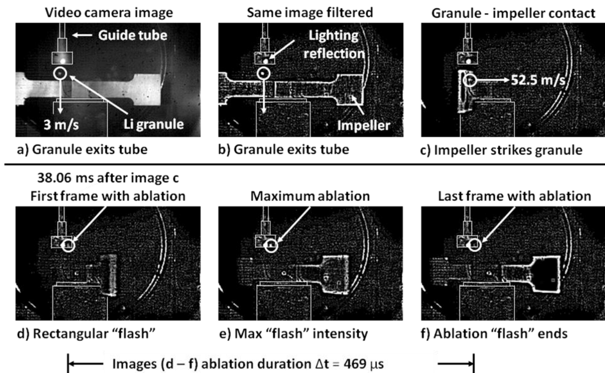
Figure 2. In this sequence of video images are shown: (a) an unfiltered view of the tenth granule falling from the guide tube at 3 m/s as the impeller was spinning with a velocity at the point of contact of 52.5 m/s, (b) The effects of applying digital filtering to (a), (c) The impeller striking the granule and imparting a horizontal velocity of \sim 52.5 m/s, (d – f) the appearance and disappearance of a rectangular "flash" on the structure at the bottom of the guide tube – indicating ablation of the granule. For this particular granule the measured TOF was 38.06 ms and the calculated granule penetration depth was 2.5 cm.
