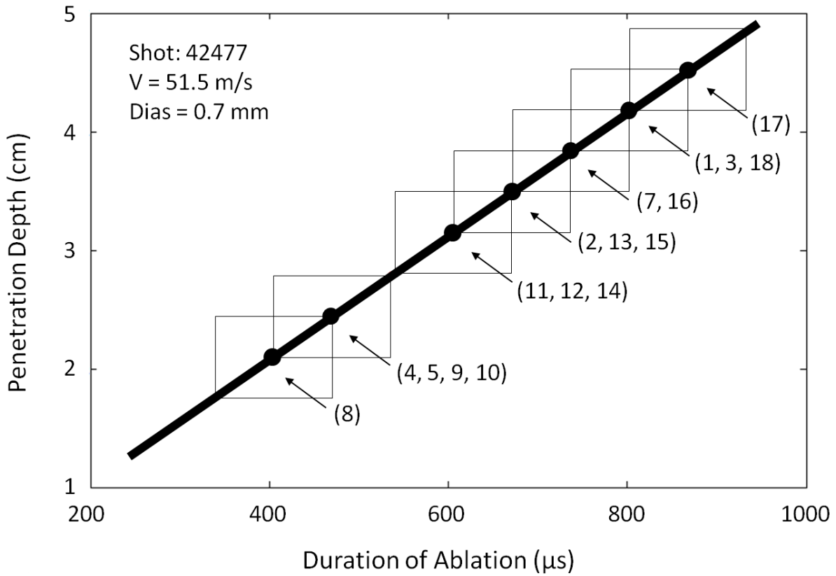
Figure 7. The apparent penetration depths of all granules injected into shot 42477. The width of each data box represents the uncertainty in the measurement of ablation time (i.e. twice the 67\mu\text{s} sampling time of the video images). The height represents the uncertainty of the penetration measurement assuming 51.5 \text{ m/s} granule velocity. The associated granule number is also shown for each of the injected granules – excluding #6. The nominal pedestal width for shot 42477 was 3 cm.
