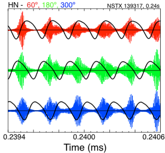
Fig. 13. Digitally filtered (1.4 - 2.0 MHz) signals from each of the three coils separated toroidally by 120°. Each color corresponds to the signal from a different toroidal position, indicated at the top of the figure. Black curves are the kink, filter from 2-30kHz.
