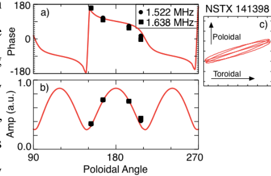
Fig. 6. Poloidal structure and polarization of the 1.52 MHz (solid circles, partially obscured by squares) and 1.64 MHz modes (solid squares); a) relative phase, b) normalized amplitude for same two modes, solid lines are fits to the data assuming a mix of standing and propagating waves, c) lissajous figures showing compressional polarization for both modes.
