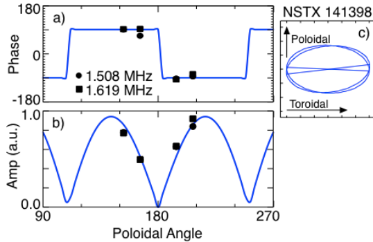
Fig. 5. Poloidal structure and polarization of the 1.51 MHz (solid circles) and 1.62 MHz modes (solid squares); a) relative phase compared to phase of standing wave for both modes, b) normalized amplitude compared to amplitude of standing wave, solid lines are fits to the data assuming a standing wave, c) lissajous figure showing mixed shear and compressional polarization for both modes.
