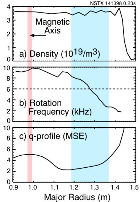
Fig. 3. a) flat density profile typical of early phase of NSTX H-modes, b) Rotation profile reaching \approx 10\text{ kHz} on axis and c) typical reversed-shear q-profile as reconstructed from MSE data.
