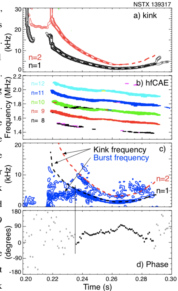
Fig. 12. a) spectrogram showing first and second harmonic of n = 1 kink mode, b) spectrogram showing hfCAE burst correlated with kink, c) spectrogram of envelope of hfCAE fluctuation amplitude, overlaid with kink mode frequencies, d) relative phase between n = 1 kink and hfCAE envelope.
