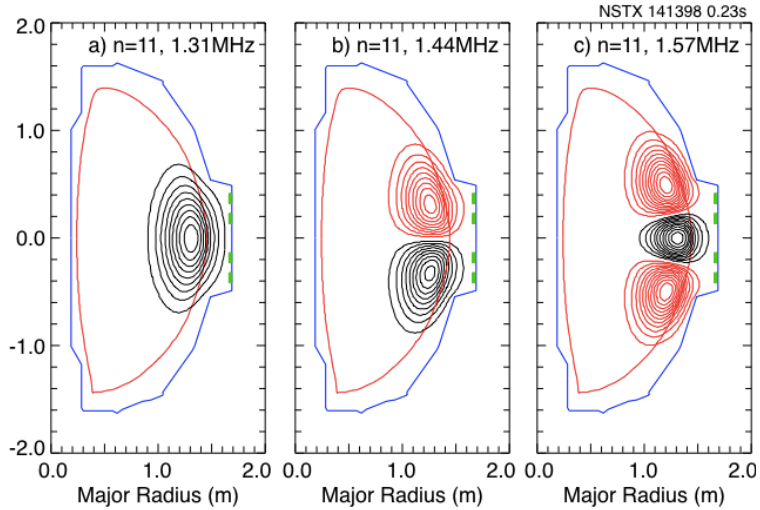
Fig. 8. Approximate eigenmodes for the first three poloidal eigenstates with n=11 . a) the lowest order n=11 poloidal eigen-state, b) the second order n=11 poloidal eigenm-state and c) the third order n=11 poloidal eigen-state.
