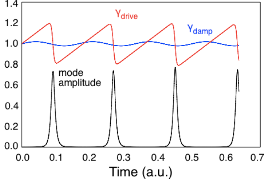
Fig. 16. Predator-Prey model simulating coupling of kink to hfCAE.
