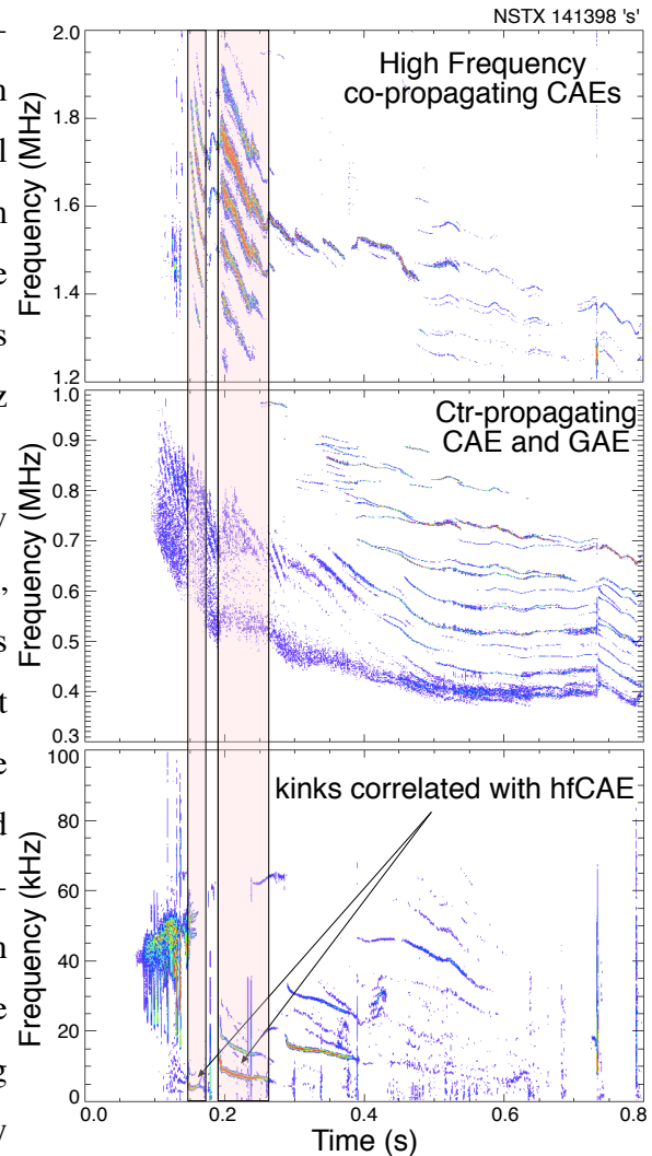
Fig. 1. Spectrograms of magnetic fluctuations; a) co-propagating, high frequency CAE, b) ctr-propagating CAE and GAE, c) rsAE, TAE and kink-like modes.
