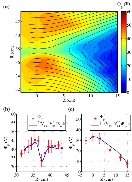
FIG. 2. (a) Measured 2-D plasma potential profile with contours of the poloidal flux \Psi . The radial potential well becomes deeper and wider downstream. (b) Radial profile of \Psi_p at Z = 0 (along the magenta dashed line in (a)). The red asterisks are the measured \Psi_p and the blue line is the radial integration of the right-hand side of Eqn. (2). Two profiles are in agreement. (c) Axial profile of \Psi_p at R = 37.5 cm (along the black dashed line in (a)). The red asterisks are the measured \Psi_p and the blue line comes from the integration of the right-hand side of Eqn. (3) along Z .
