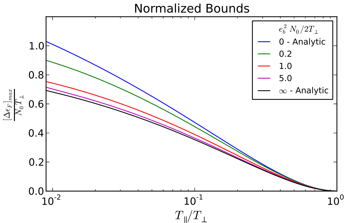
Figure 1. The normalized nonlinear thermodynamic bound on the change in field perturbation energy as a function of T_{\parallel}/T_{\perp} for bi-Maxwellian distributions described by Eq. (40) for several values of the dimensionless parameter e_b^2 N_0/2T . The bounding curves in the emittance-dominated limit ( e_b^2 N_0/2T \rightarrow 0 ) and space-charge-dominated limit ( e_b^2 N_0/2T \rightarrow \infty ) are obtained from the analytical estimates in Eqs. (39) and (36), respectively.
