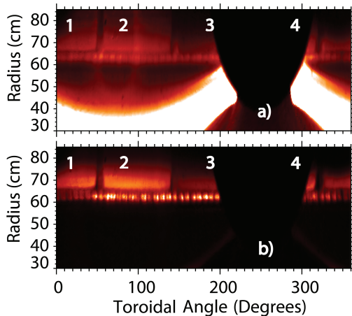
FIG. 4. a) D- \alpha and b) Li I emission with heated LLD.
