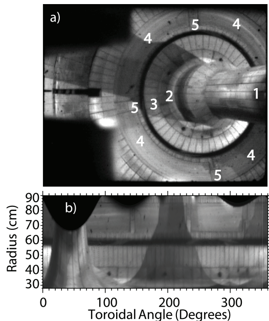
FIG. 1. a) Bay E lower divertor view: 1) center stack, 2) and 3) 1 st and 2 nd row of graphite tiles, 4) LLD, 5) diagnostic graphite tiles; b) polar remapping of Bay E view.
