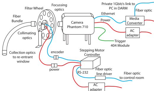
FIG. 2. Schematic of camera setup.
