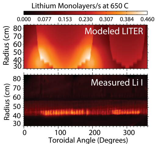
FIG. 3. Simulated fresh lithium coatings thickness (top) and measured Li I brightness from the lower divertor (bottom).
