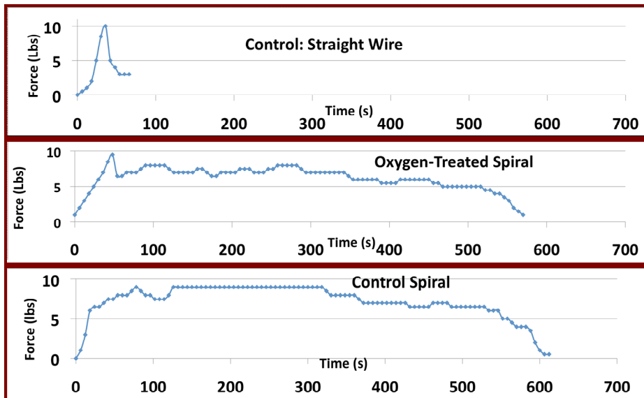
Fig. 6. A comparison of the oxygen-treated spiral response to applied force and the response of a straight electrode.
