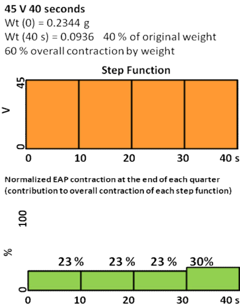
Fig. 10. Applied voltage step function experiments.
