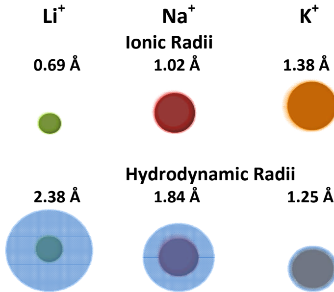
Fig. 12. Ionic and hydrodynamic radii for lithium, sodium and potassium Group 1 cations.
