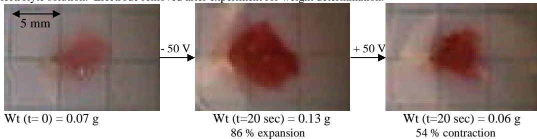
Fig. 2. Expansion-contraction cycle. Note: Red dye added to (uncoated) EAP to improve visualization.
