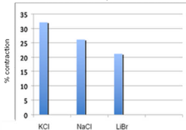
Fig. 13. Contraction of PMA based EAPs for three different electrolyte systems.
