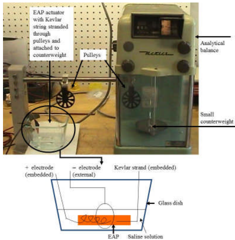
Fig. 8. Isometric mechanical testing set-up.
