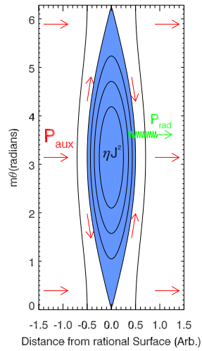
Figure 1: Representation of single lobe of a magnetic island schematically showing the heat flow from the auxiliary heating around the island (red arrows), the resistive heating inside the island (blue area), and the radiation losses from within the island interior (green arrow)
