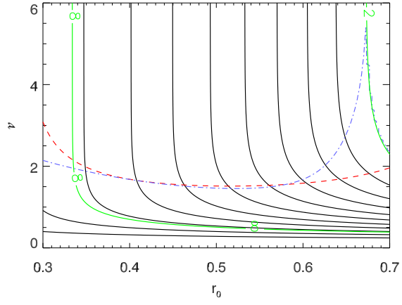
Figure 3: Contour plot of the total plasma current (black) as a function of the profile parameters \nu and r_0 . Also shown in the plot are the contour of the current profile peaking at the density limit as given by Equation 6 and the best fit contour of the quantity from Equation 8
