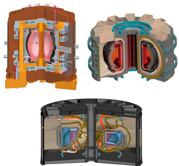
Fig. 1. Pilot plant configuration designs based on (clockwise from top left) spherical torus (ST), advanced tokamak (AT), and compact stellarator (CS). Not to scale.
