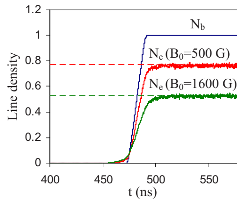
FIG. 13. (Color online) Time evolution of the ion and electron line densities at the center of the magnetic solenoid ( z=60 cm) obtained using the LSP simulations. The blue curve shows the ion beam line density, and the red and green curves show the electron beam line density for the cases where the maximum values of the solenoidal magnetic field are B_0=500 G and B_0=1600 G, respectively. The corresponding horizontal dashed lines illustrate the solutions to Eq. (22) with r_w/r_b=3.8 .
