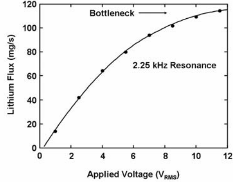
Fig. 4 Li powder data: Each point represents the mass dropped during a 1s constant resonant sinusoid.
