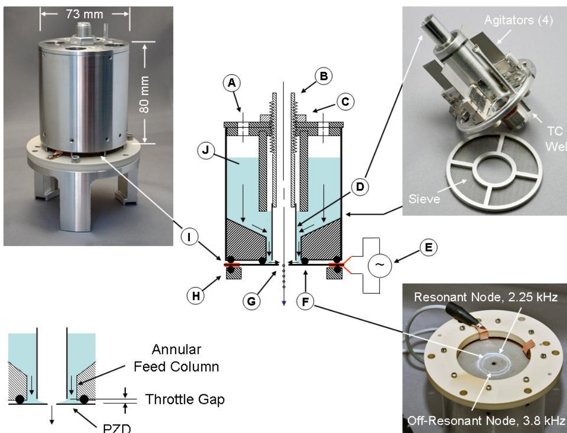
Fig. 2 The dropper/injector: Details A – J are described in the text. An assembled dropper appears at upper left. An inverted throttle assembly is displayed at upper right. The agitators, thermocouple well and sieve (see text) are not represented in the schematic. The throttle gap and AFC – also explained in the text – appear at lower left. At lower right a resonant (0, 2) node can be seen by the accumulation of glass beads on an unsupported PZD (i.e. with particle containment O-ring removed from below). Also seen is a smaller non-resonant node previously driven at equal voltage but higher frequency causing lower amplitude of vibration. Redundant electrode tabs also appear.
