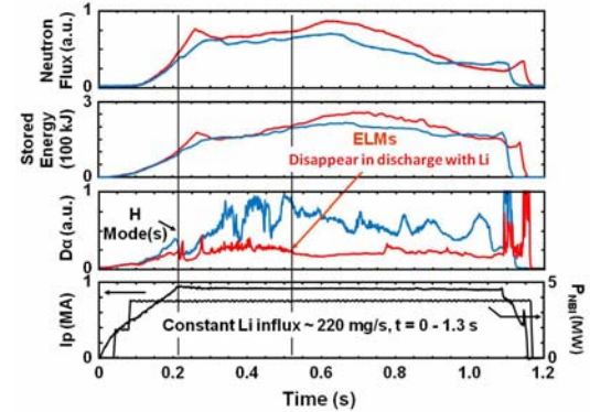
Fig. 6 Neutron rates, stored energies and D \alpha emissions of H-Mode discharges with (red) and without (blue) Li aerosol injection. Common current and NBI powers are shown in black.
