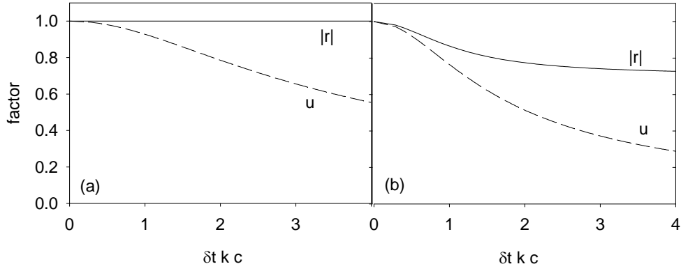
Figure 2: The amplification factor |r| and the effective normalized wave velocity u \equiv \omega \delta t / \sqrt{D / \rho_0} \sim \omega / kc , where k and c are the wave number and wave velocity associated with the operator \mathbf{G} with eigenvalue \lambda = -\rho_0 k^2 c^2 . (a) for the Caramana method ( \phi = 1, \theta = \frac{1}{2}, \alpha = \theta^2 ), and (b) for the split \theta -implicit method ( \phi = \frac{1}{2}, \theta = \frac{1}{2}, \alpha = -\frac{1}{2} )
