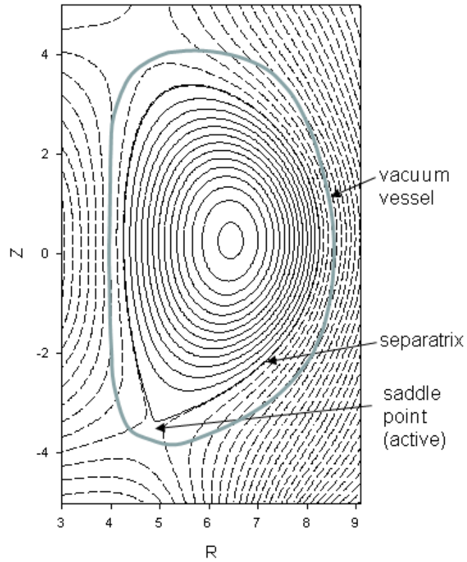
Figure 1: In a tokamak, the equilibrium plasma is axisymmetric. Magnetic flux surfaces are closed interior to the separatrix and open exterior to it. Plasma is surrounded by a metallic vacuum vessel.
