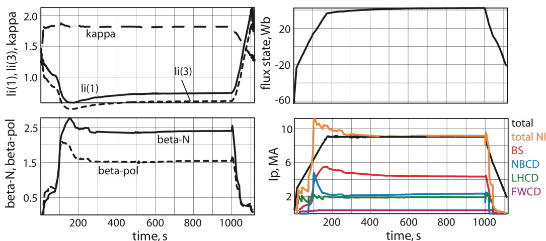
Figure 1. Time histories of the plasma current contributions, normalized and poloidal beta, flux state, li and elongation for a steady state discharge simulation utilizing NB, LH, and IC. The simulation is run to 1000s and then rampdown is initiated.
