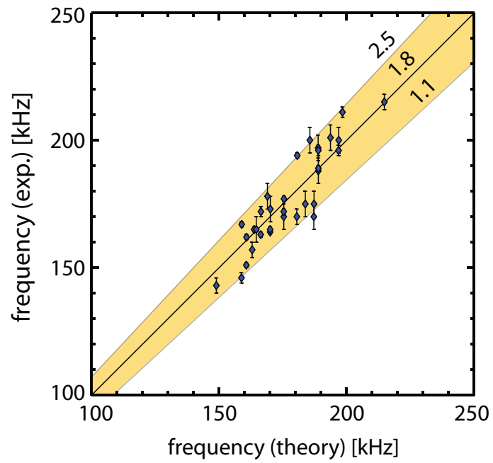
Figure 9: The collection of minimum frequency data is compared to Eq. 4. The analysis finds a best-fit value of the ion adiabatic index ( \gamma_i ) of approximately 1.8, a result very close to the theoretical prediction of 7/4 .
