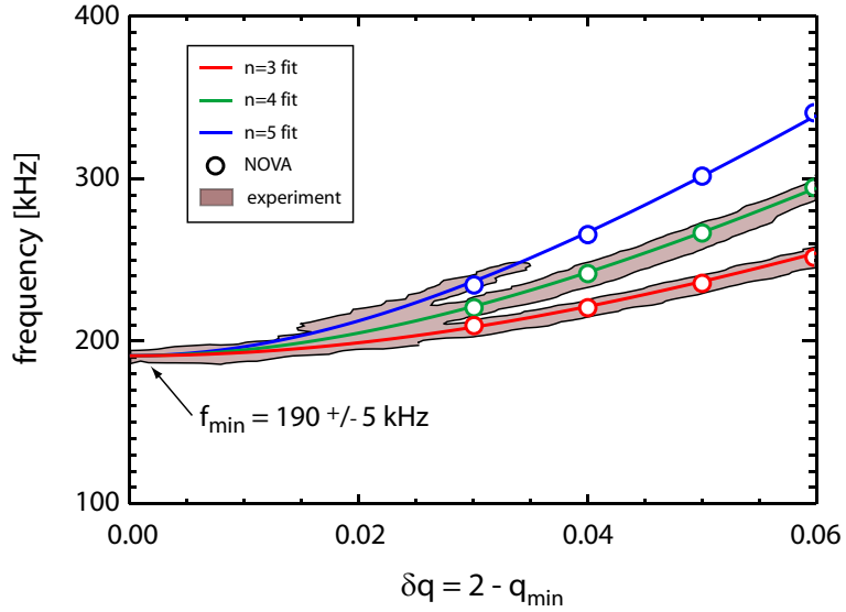
Figure 6: (color online) While NOVA cannot directly calculate f_{min} on account of the larger continuum interaction which distorts the eigenmodes, it can produce viable solutions in the neighborhood of f_{min} . Using an analytic approximation (colored lines) the NOVA frequencies (circles) are extrapolated to a common minimum frequency, which agrees well with the experimental measurements of the minimum frequency (shaded region).
