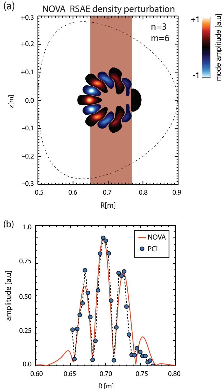
Figure 4: (color online) (a) The two dimensional density perturbation calculated by NOVA for the n = 3 mode near 140 msec identified in Fig. 3. The shaded area indicates the PCI viewing region. (b) The synthetic PCI data is compared to the experimental data, showing overall good agreement between the structures. The nodes in the structure arise from cancelation of positive and negative density perturbations.
