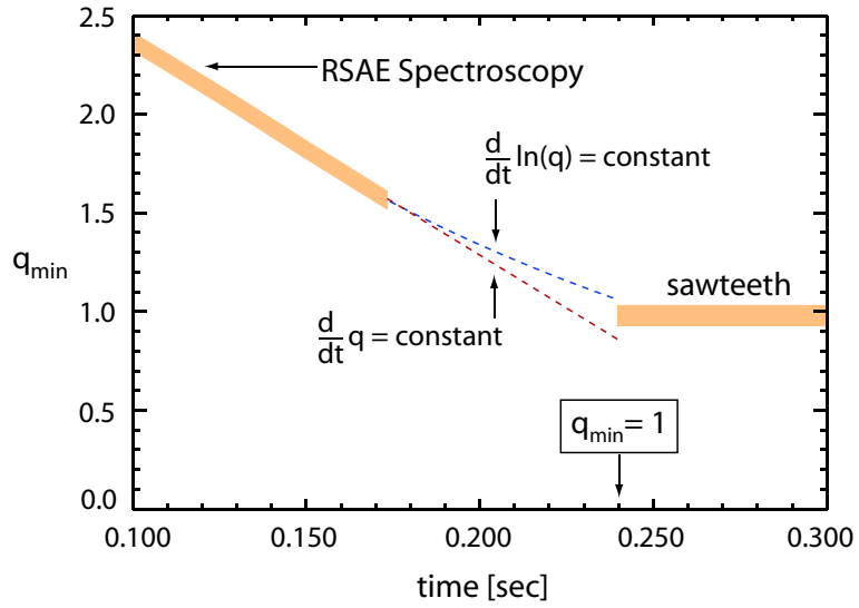
Figure 5: (color online) MHD spectroscopy of the RSAEs (100-180 msec) and the presence of sawteeth (240+ msec) provide limits for the evolution of q_{min} during the current ramp. Extrapolation of the inferred q_{min} trajectory to the time of sawteeth is seen to lie between the curves d_t q = \text{constant} and d_t \ln q = \text{constant} .
