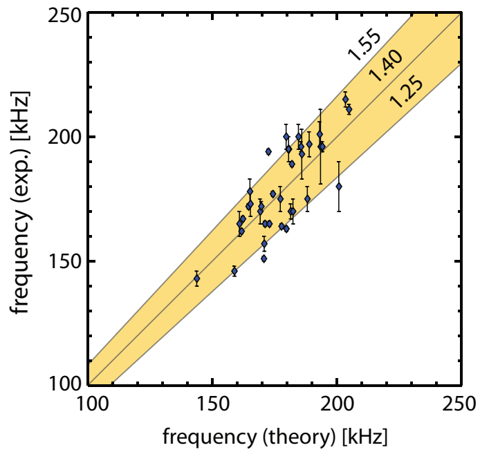
Figure 8: The collection of minimum frequency data is compared to the empirical NOVA scaling of the minimum frequency to derive \gamma . This analysis finds a best fit \gamma of 1.40 \pm 0.15 , with the error bars resulting from the uncertainties in the experimental temperature profiles.
