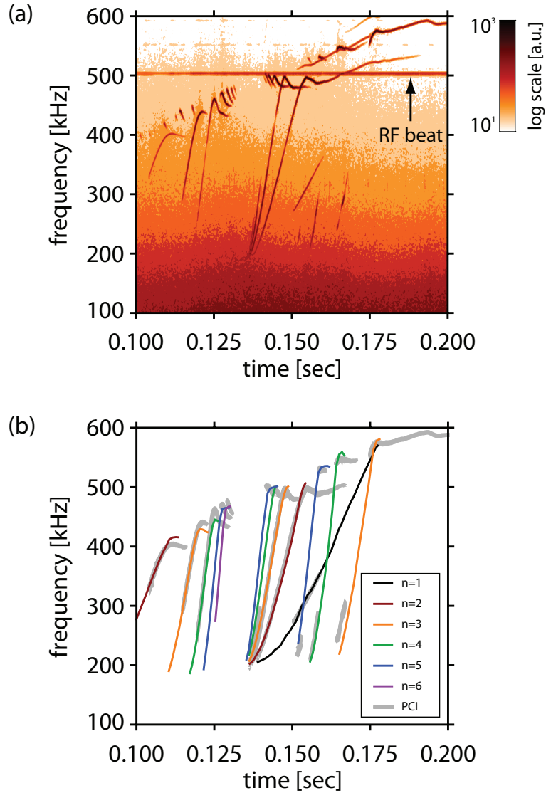
Figure 3: (color online) (a) Composite spectrogram averaged over all 32 channels of the PCI diagnostic. RSAEs are present during the time range 100-180 msec, with a grand cascade occurring at approximately 130 msec which identifies the entrance of the q = 2 surface to the plasma. (b) RSAE spectra calculated by NOVA (color) as the q profile is decreased are compared to experimental PCI measurements (gray), allowing the evolution of q_{min} to be determined.
