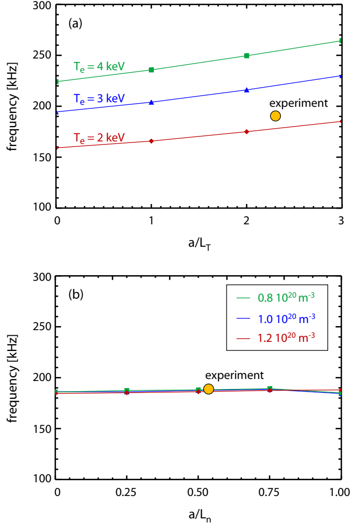
Figure 7: Parameter scans in NOVA show that the minimum RSAE frequency has (a) a strong temperature dependence and weaker temperature gradient dependence and (b) no significant dependence on density and density gradient. The gradient scans were performed with the value of the profile held constant at the peak of the eigenmode. For the experimental data shown in Fig. 6 the electron temperature near q_{min} is about 2.3 keV, in good agreement with an interpolation of the scaling studies shown here.
