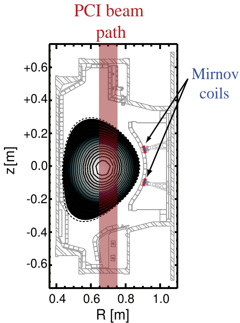
Figure 2: (color online) Cross section of the Alcator C-Mod tokamak showing the position of the PCI beam path and the poloidal location of the two sets of Mirnov coils.
