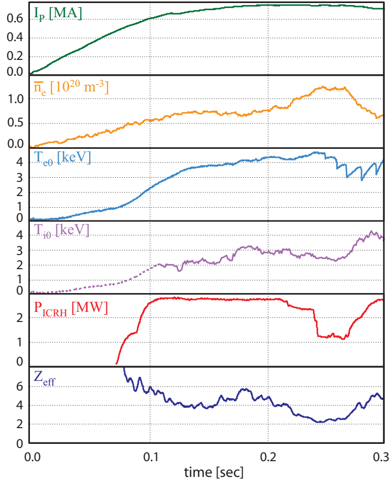
Figure 1: (color online) Overview of plasma parameters corresponding to the experiment examined in Fig. 3.
