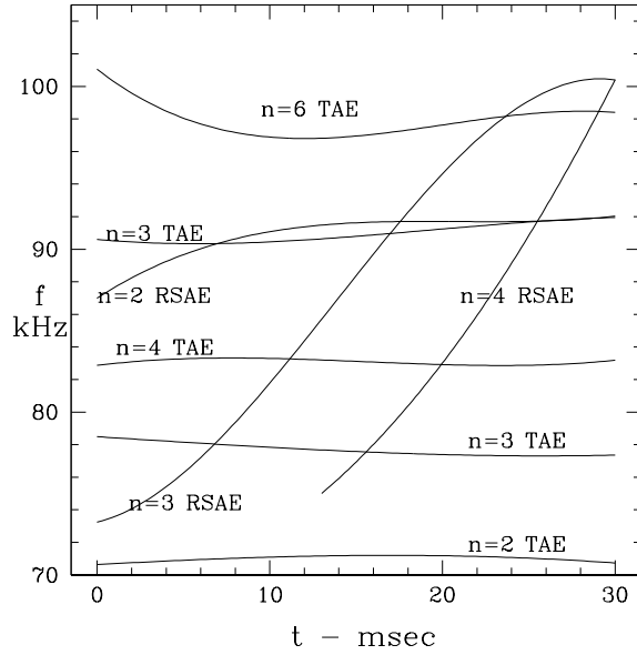
FIG. 5: Time dependence of the modes in the spectrum
