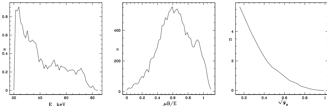
FIG. 3: Initial Beam distribution in energy, pitch, and flux surface.
