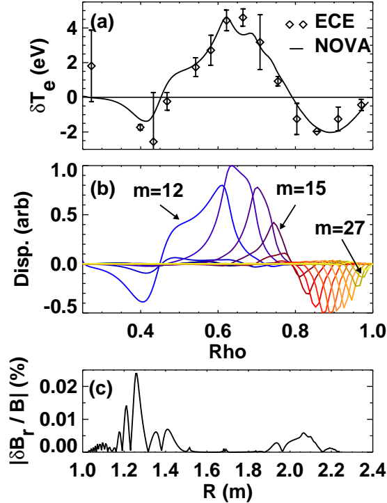
FIG. 4: (color online) (a) Synthetic ECE diagnostic prediction (solid) using NOVA calculated f = 78 kHz global TAE overlaid with ECE measurements (diamonds). NOVA prediction scaled by single constant to match ECE data. (b) Poloidal harmonics comprising TAE from panel (a). (c) Calculated radial component of magnetic field fluctuation along device midplane (vs. major radius) using amplitude obtained from comparison with ECE data[5].
