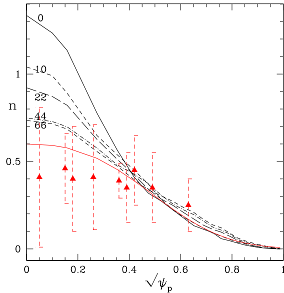
FIG. 7: Beam modification due to modes, including beam slowing down and continuous injection, with time shown in msec. Shown also are experimental data points from reference [6].
