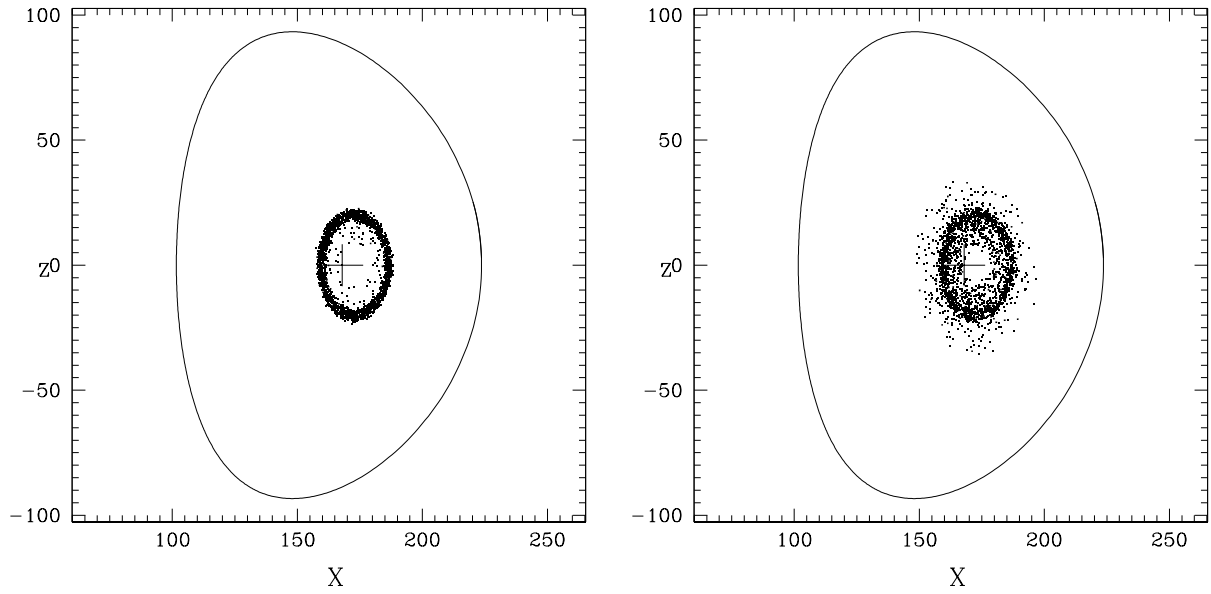
FIG. 6: Particle distribution after 7 msec, all launched at the outer midplane with pitch \lambda = 0.6 with random toroidal angle in the presence of the full spectrum of modes, but with no collisions. Amplitudes of dB/B \simeq 1.2 \times 10^{-4} , (a), and dB/B \simeq 1.6 \times 10^{-4} , (b)
