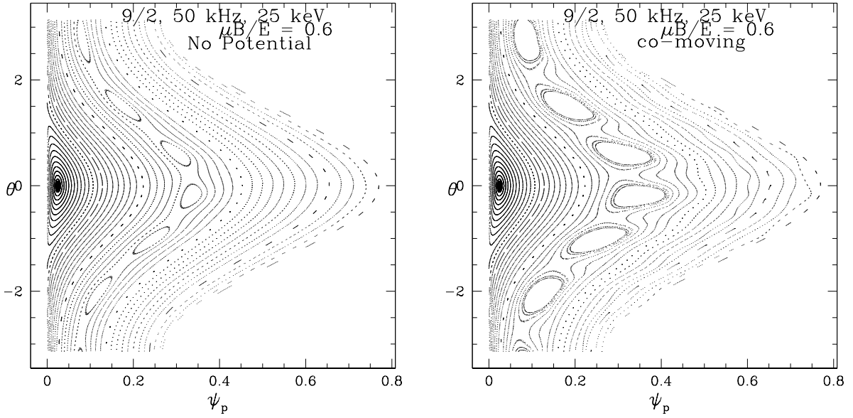
FIG. 2: Kinetic Poincaré plots for mode m/n = 9/2 , showing the effect of the potential on 25 keV beam particles for a 50 kHz mode.
