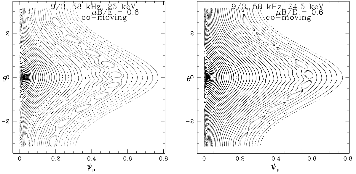
FIG. 1: Kinetic Poincaré plots for mode m/n = 9/3 , showing energy dependence of the m' = 10 resonances. Shown are the resonances for a 9/3 perturbation on particles of 25 \text{ keV} and 24.5 \text{ keV} .
