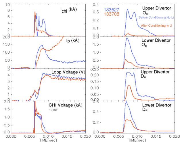
Figure 3. This shows two CHI initiated discharges. The discharge with the curves indicated in blue are from a discharge taken early in the CHI campaign, while those in red are from a discharge after discharge cleaning and with the benefits of Li evaporation
