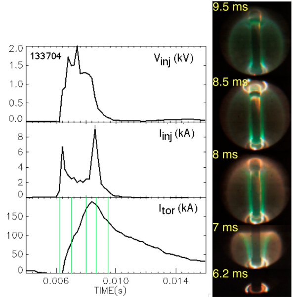
Figure 2. On the left are shown the CHI injector voltage and current and the plasma current versus time for a CHI only discharge. On the right are fast color camera images of the plasma taken at the times marked by the green bars in the left figure as it grows up from the bottom after breakdown at about 6 ms. Note that the ratio of I_{inj}/I_{ptor} reaches well over 50 before an absorber arc occurs at about 8.5 ms.
