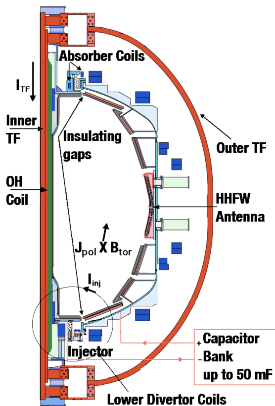
Figure 1. This cross-sectional view of NSTX shows the field direction for the initial magnetization state of a transient CHI discharge. Gas is introduced into the volume below the injector gap (lower divertor gap) when the capacitor bank is fired.
