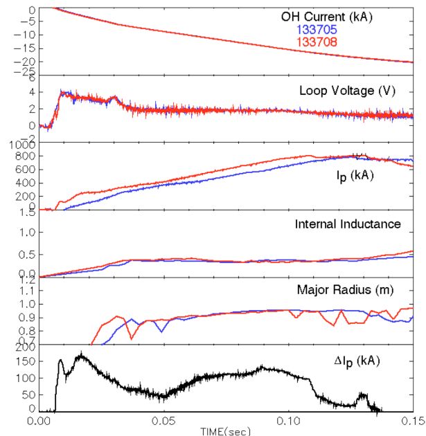
Figure 4. Comparison of discharges taken with CHI coupled to inductive ramp-up in red and an with induction only in blue. The discharges had identical OH current programming and thus similar Loop Voltage histories. The CHI plus ohmic clearly has higher current until a reconnection event occurs as the loop voltage is reduced. The similar internal inductance and major radius of the plasmas indicate that the increased plasma current shown in the bottom frame is due to a real flux savings with CHI.
