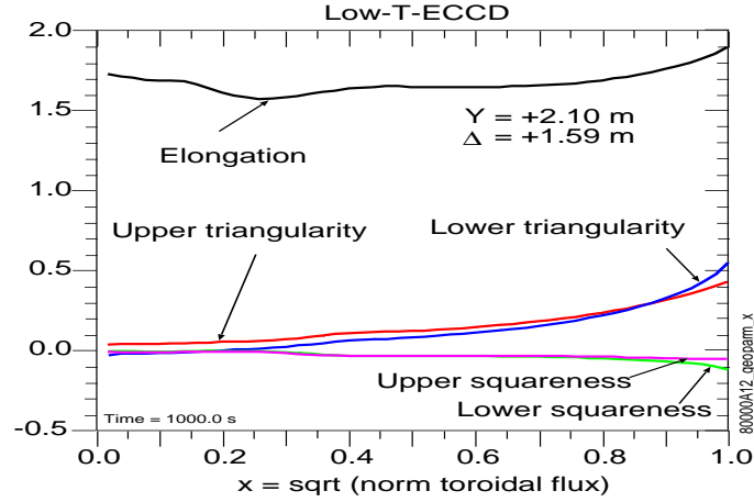
FIG. 8: (Color online) Profiles of the elongation, upper and lower triangularities, and upper and lower squarenesses for one of the Low-T-ECCD mode aimings with footprint height Y=+2.10 m relative to the vessel midplane, and \Delta = +1.59 m relative to the plasma magnetic axis.
