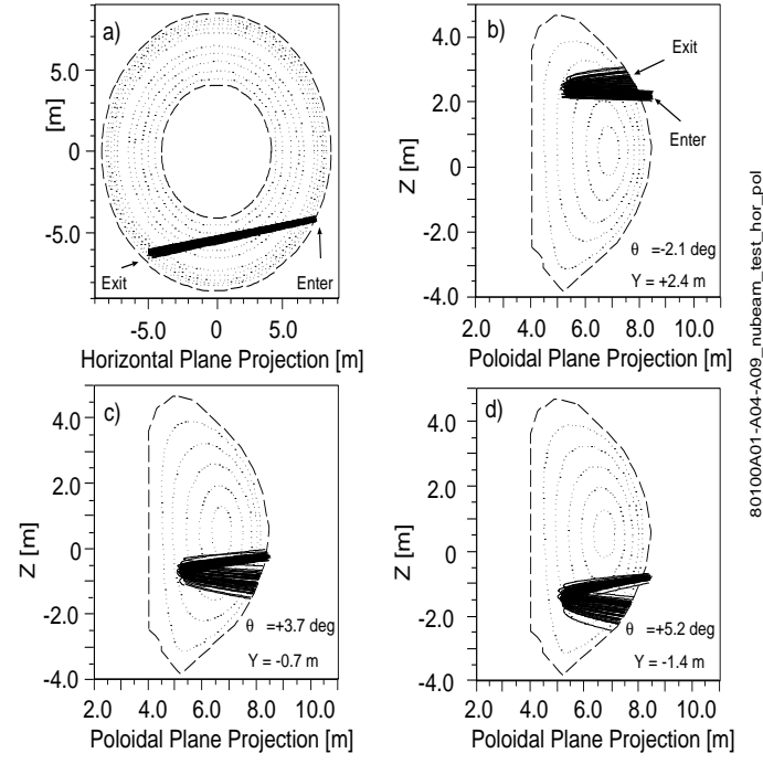
FIG. 5: Trajectories on NNBI neutrals with three different steering angles: a) Horizontal view showing co-injection (parallel to I_p ); b) high steering with neutrals clustered around a height Z near +2.40 m at the minimum tangency radius; c) clustered near -0.68 m; d) clustered near -1.40 m. The beam system and port ducts have not been finalized. The extreme upper and lower steerings are not compatible with the preliminary designs of the beam ducts unless the injectors are raised or lowered from their heights assumed here. The heights Y relative to the plasma magnetic axis are indicated.
