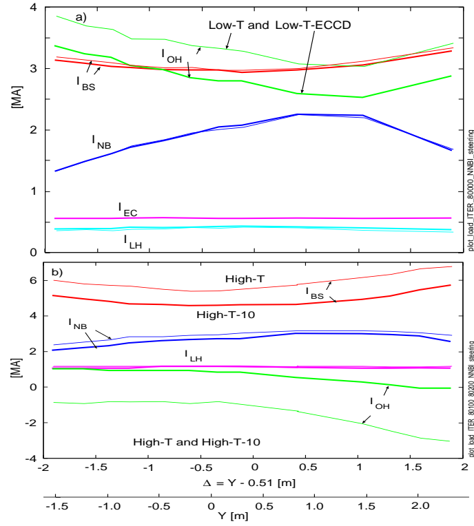
FIG. 11: (Color) Total currents for the a) Low-T (thin) and Low-T-ECCD (thick) and b) High-T (thin) and High-T-10 (thick) modes versus the footprint height and \Delta = footprint height minus the height of the magnetic axis. The right-left asymmetry of I_{NB} and I_{BS} in \Delta is caused by the helicity of the magnetic field.
