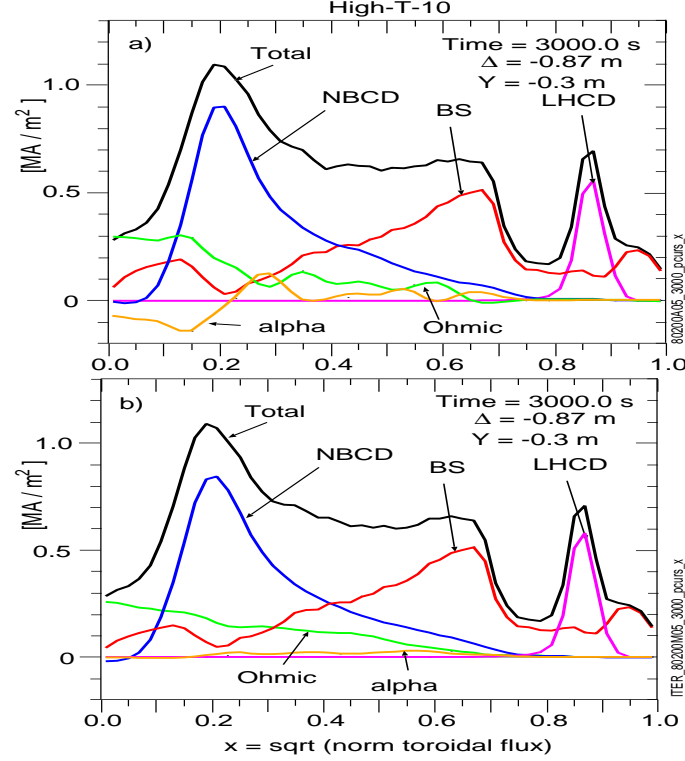
FIG. 18: (Color) Current profiles for one of the aimings from the High-T-10 mode. The number of Monte Carlo samples are varied to compare effects of noise. In a) 5000 beam and 1000 alpha Monte Carlo particles are used. In b) 50,000 beam and alpha Monte Carlo particles are used. The profile of the alpha-driven current (analogous to the beam-driven current but from an isotropic DT source) fluctuates in time considerably more in the first case. The time-averages of the alpha-driven currents peak near 0.02 \text{ MA/m}^2 in both cases.
