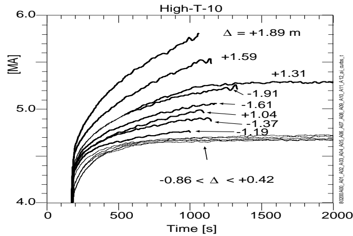
FIG. 12: Evolution of the total bootstrap current for various aimings with the High-T mode.
