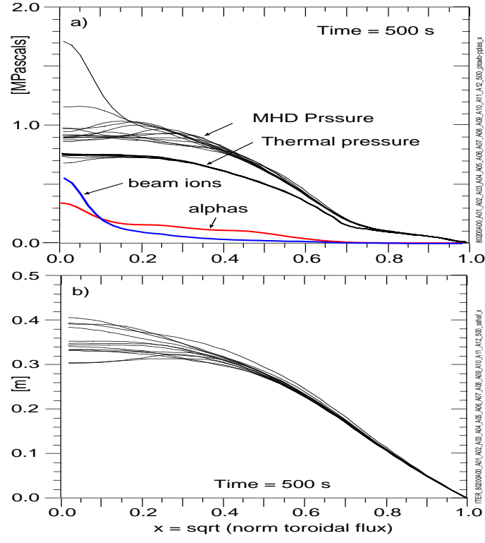
FIG. 7: (Color online) a) Profiles of the thermal and MHD pressure profiles defined in equation (1) for the High-T-10 mode with various NNBI aimings. The contributions of the beam ions and alphas for one of the aimings ( Y=+0.39 m, \Delta \equiv Y - 0.51 m) are shown. The beam contribution varies with the aiming as discussed below, whereas the alpha contribution does not vary. b) Profiles of the Shafranov shifts.
