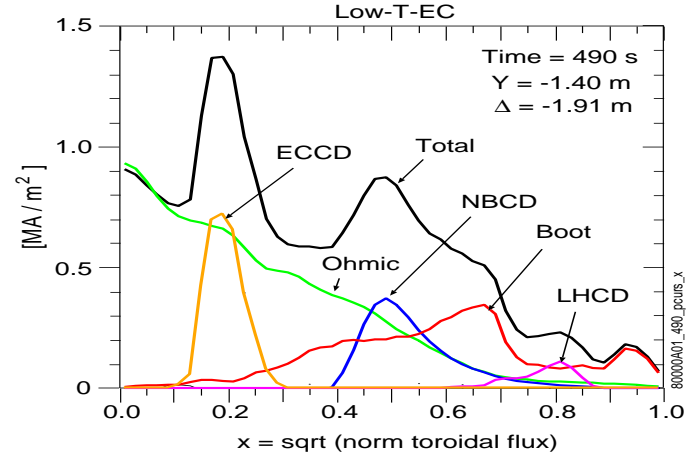
FIG. 16: (Color) Current profiles for one run from the Low-T-ECCD mode.
