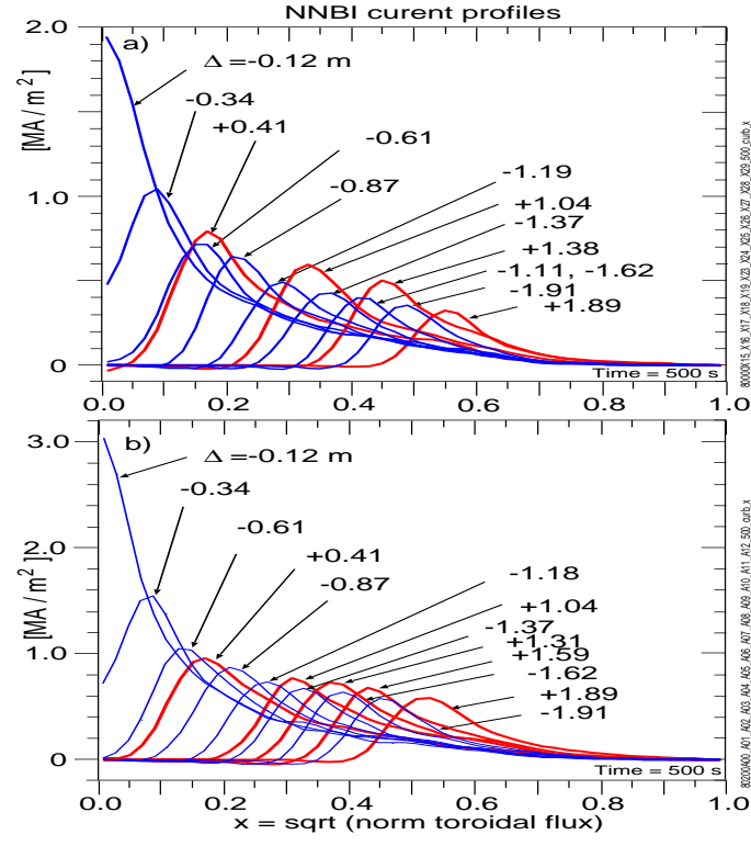
FIG. 13: (Color) Profiles of the NNBI current drive for various aimings of the a) Low-T and Low-T-ECCD modes, and b) High-T and High-T-10 modes. The profiles with aiming above the magnetic axis ( \Delta positive) are colored red, and those below colored blue.
