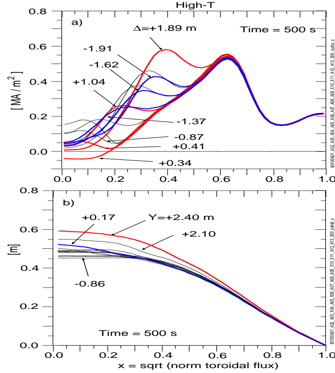
FIG. 14: (Color) Profiles with different aimings at 500 s for the High-T mode of a) the bootstrap current, and b) the Shafranov shift. The profiles of the bootstrap current have been smoothed over an interval of x=0.1 .
