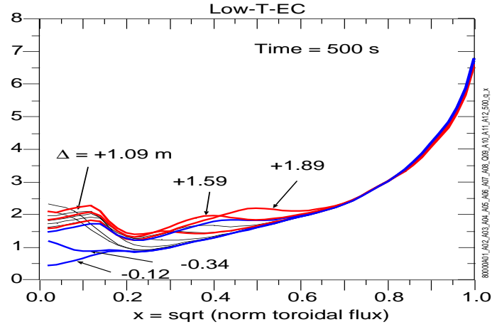
FIG. 20: (Color) Profiles of q at 500 s from the Low-T-ECCD mode.
