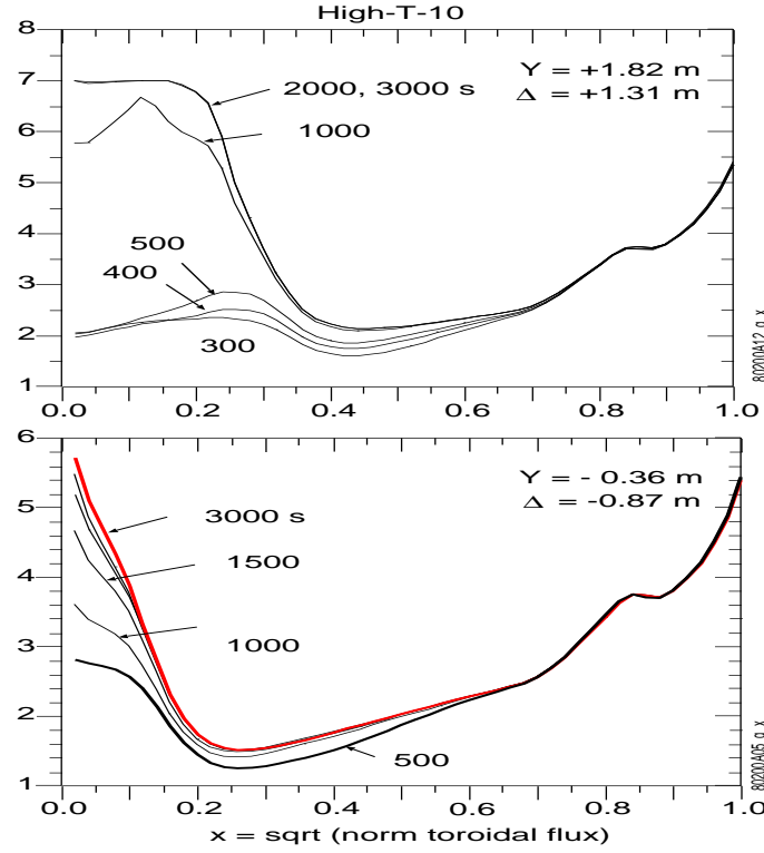
FIG. 22: (Color online) Evolution of q from two of the High-T-10 mode aimings.
