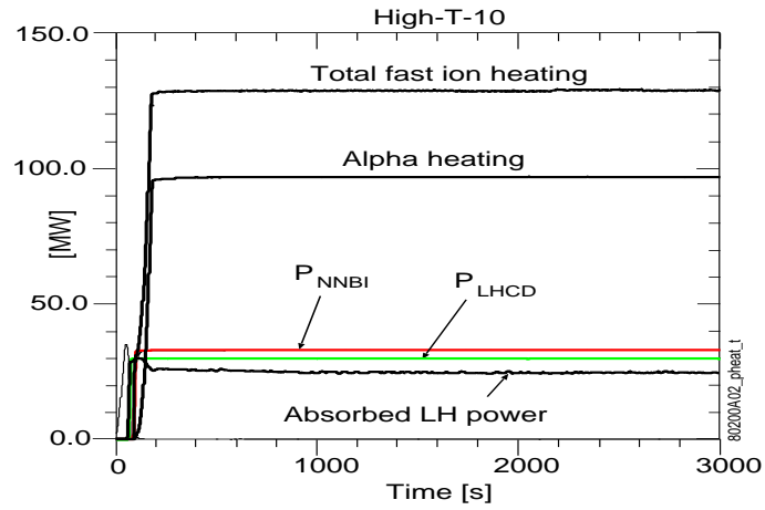
FIG. 6: (Color online) Heating for one of the High-T-10 mode aimings.
