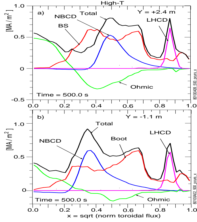
FIG. 17: Current profiles for two aimings from the High-T mode.
