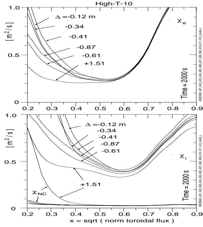
FIG. 25: Profiles of the electron, ion and neoclassical heat conductivity for the High-T-10 mode at 2000 s. The profiles have been smoothed in x . Three of the predictions have central q greater than unity.
