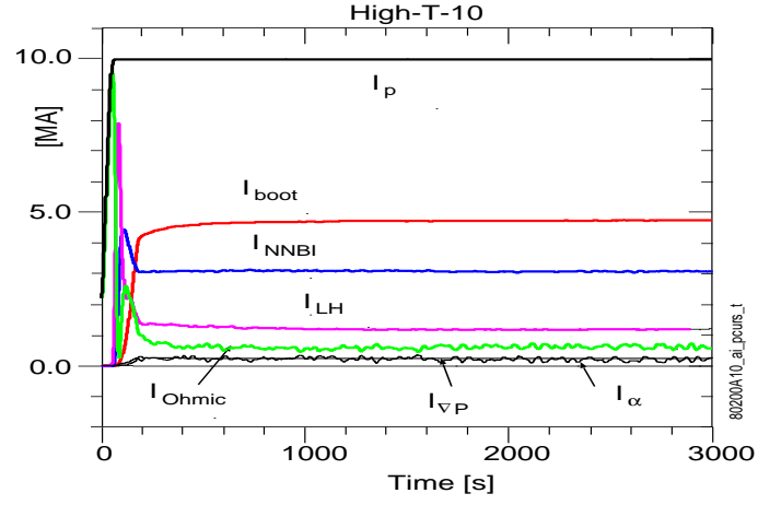
FIG. 3: (Color) Plasma currents for one of the High-T-10 mode aimings. The total is assumed to be 10 MA and the other currents are computed. Besides the dominant bootstrap, beam, and Lower Hybrid currents, small contributions from currents driven by the gradient of the pressure and the fast alphas are calculated.
