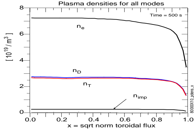
FIG. 4: (Color online) Assumed flat top density profiles. The n_e profile is assumed and the others are computed. A single impurity ion is assumed with Z=6 , A=12 , and Z_{eff}=2.17
