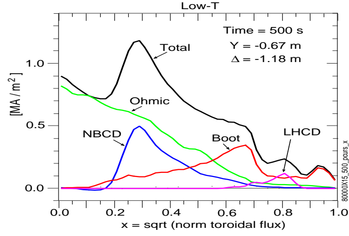
FIG. 15: (Color) Current profile for one case of the Low-T mode.
