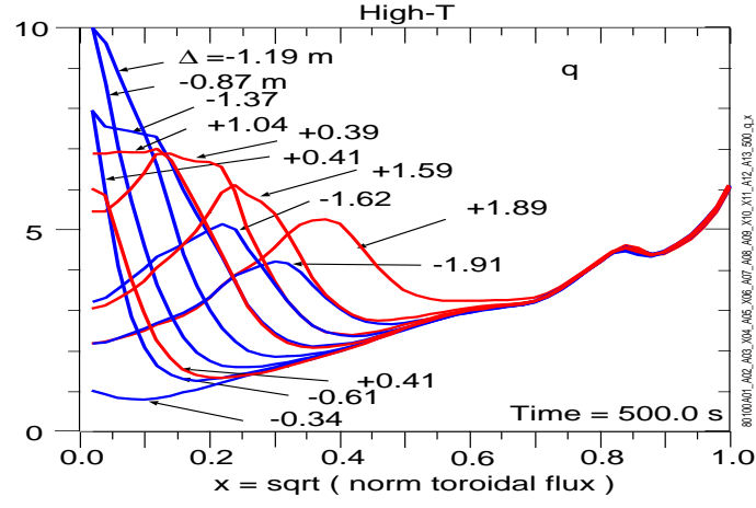
FIG. 23: (Color) Profiles of q from the scans of High-T mode at 500 s.
