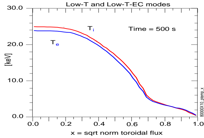
FIG. 2: (Color online) Assumed flat top temperature profiles for the Low-T and Low-T-ECCD modes.
