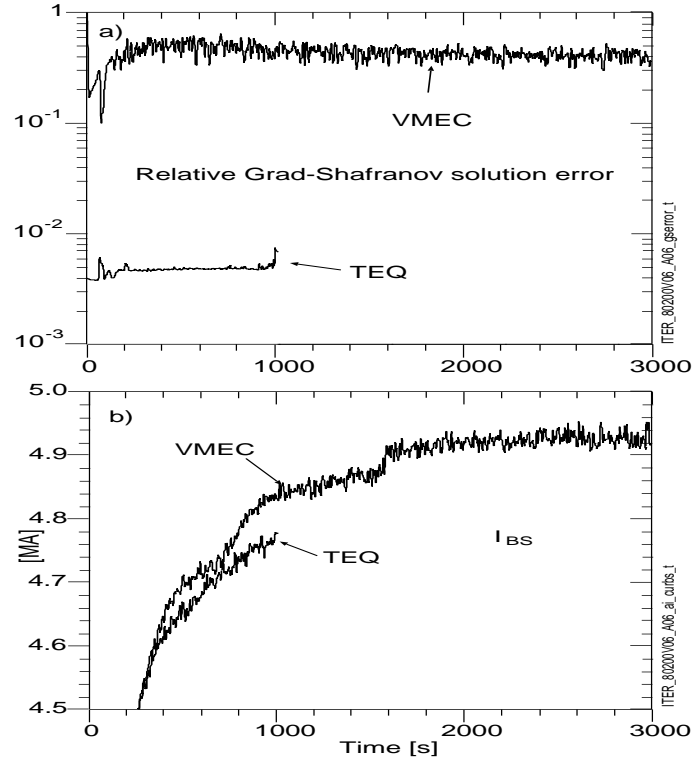
FIG. 9: Comparison of results from two runs identical but for the choice of the Grad-Shafranov solvers VMEC and TEQ showing a) the relative errors of the Grad-Shafranov equation solutions, and b) the calculated total bootstrap current. The relative error is defined as the surface-averaged magnitude of the difference between the left and right side of the Grad-Shafranov equation normalized by the total. The run using TEQ crashed at 1005 s whereas the run using VMEC completed to the specified 3000 s.
