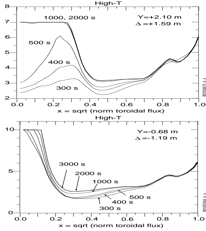
FIG. 21: Evolution of q profiles for two aimings from the High-T mode. For the case with high aiming, a current hole develops by 1000 s. The case with low aiming the current hole persists.
