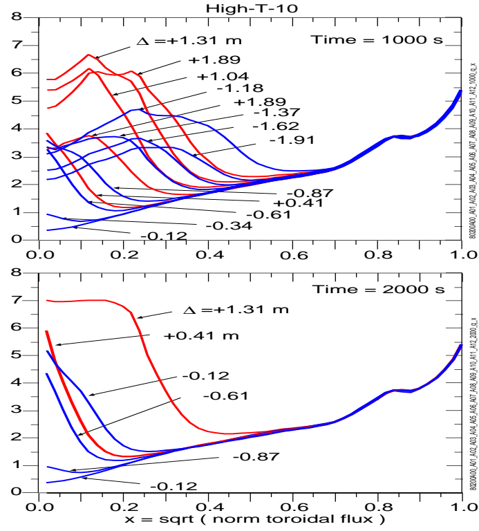
FIG. 24: (Color) Profiles of q from the High-T-10 mode at 1000 and 2000 s. A current hole develops in the run with \Delta = 1.31 m after 1000 s, and so the value of q is limited to 7.0.
