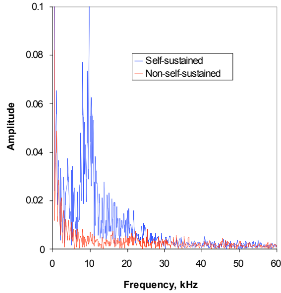
Fig. 11. Frequency spectrum measured for the self-sustained and non-self-sustained regimes of the 2.6 cm CHT operated in the direct (a) and cusp (b) magnetic field configurations.
