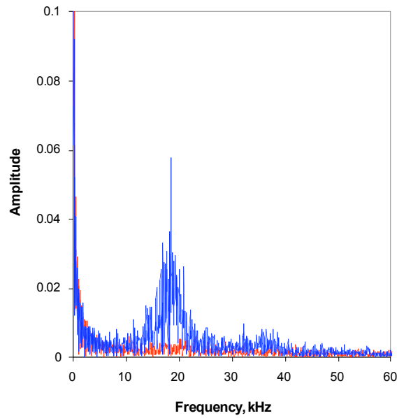
Fig. 10. The oscilloscope traces of the discharge current oscillations (a) and corresponding frequency spectrum (b) for self-sustained and non-self-sustained regimes of the annular HT.
