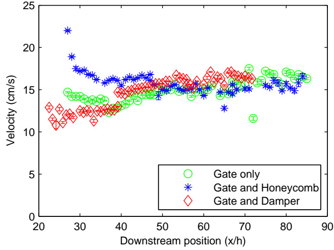
FIG. 4: The downstream velocity profile for the three flows. Measurements were taken at the mid-height of the flow along the center of the channel.
