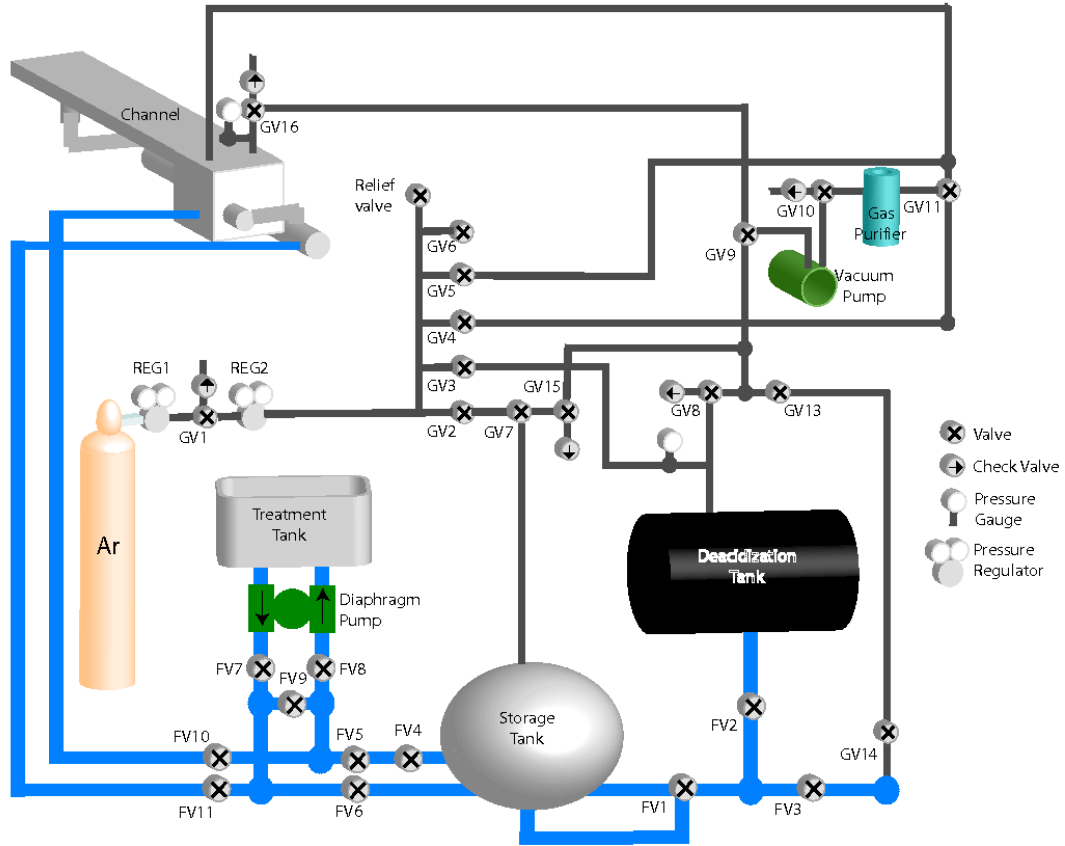
FIG. 2: A schematic of the pneumatic transfer system used to convey the liquid metal alloy between a storage tank and the experiment.
