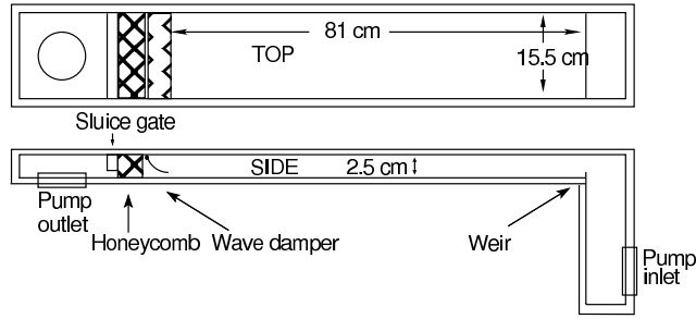
FIG. 1: A schematic of the channel used in the experiment showing the locations of the sluice gate, honeycomb, and wave damper in the channel.
