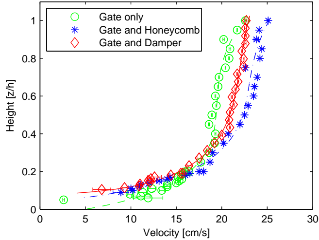
FIG. 5: A plot of the vertical velocity profile in the developed flow at x/h = 78 for the three different flows. The measurement height is normalized to the flow height.
