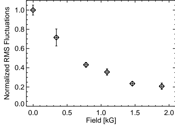
FIG. 8: Damping of cross-channel surface slope fluctuations with applied magnetic field. The fluctuation amplitudes, as quantified by the average standard deviation of the laser spot positions, is normalized to the fluctuations with no applied field. The CCD camera is oriented to maximize the resolution in the cross-channel direction.
