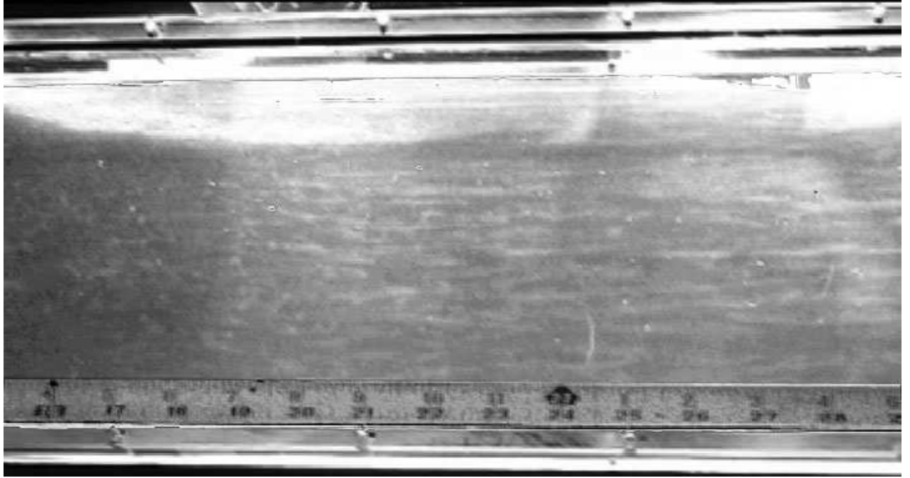
FIG. 3: Flow visualization of longitudinal vortices. The addition of a rheoscopic fluid reveals long stream-wise vortices.
