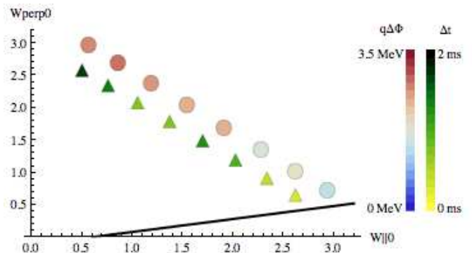
FIG. 3: Numerical simulation of alpha channeling. The circles indicate the amount of energy channeled into the radial potential. The triangles indicate the loss time. Both circles and triangles refer to the same set of alpha particles born at 3.5 MeV; their position indicates the ratio W_{\perp 0} / W_{\parallel 0} at birth. Each point is the average of 20 single-particle simulations.
