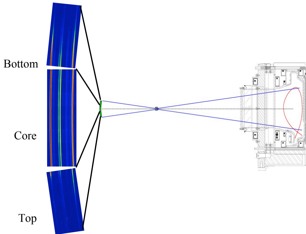
FIGURE 7. Spatially resolved He-like argon spectra from Alcator C-Mod
