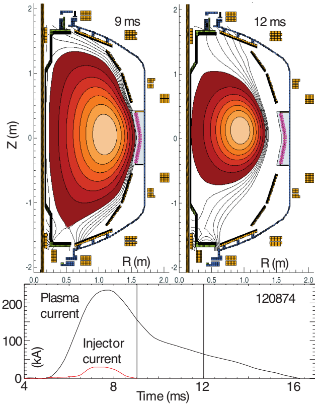
FIG. 3 (color). Equilibrium reconstructions show the shape evolution of the CHI produced plasma in response to decaying current, which is further evidence of decoupling from the injector leaving behind an inductively decaying plasma. In this discharge the increase in I_{inj} around 7.5 ms is due to the presence of an absorber arc. Overdriving the injector by using a larger capacitor bank (45 mF, charged to 1.8 kV) caused a large amount of unused capacitor bank energy to be dissipated as an absorber arc, which probably contributed to an increase in the resistivity of these yet unoptimized discharges.
