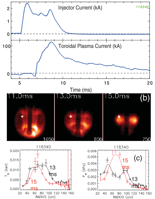
FIG. 2 (color). Shown are (a) I_p and I_{inj} traces, (b) fast camera images, and (c) the electron temperature and electron pressure profiles, at 13 and 15 ms from a CHI discharge in NSTX. The highest measured electron temperatures (not shown here) in transient CHI discharges during the closed flux phase was 30 eV. In this discharge about 2 kA of I_{inj} produces 120 kA of toroidal current resulting in a current multiplication of 60. The best attained current multiplication (not shown here) was 70. During these discharges, the NSTX CS was disconnected from its power supply. The small bright glow is light from a tungsten filament. The images at 11 and 13 ms show an elongated dark region, which is surrounded by a brighter region, like usual tokamak photos. The darker region is probably where most of the toroidal current flows, but because the neutral interaction is strongest in the edge region and because the image brightness is a function of neutral density and electron temperature, the brightness or darkness cannot be directly correlated to the electron current density in these visible camera images. Such images are used as control room diagnostics for discharge development. It is also useful to note that an absorber arc has not been produced in this discharge.
