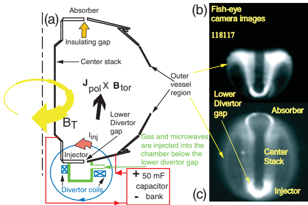
FIG. 1 (color). Shown are (a) the NSTX machine components used for CHI start-up in NSTX and fast camera fish eye images showing (b) discharge evolution from near the injector region and (c) later during the discharge. The bright region at the top of image (b) is the top of the CHI plasma that has extended to approximately the middle of the vessel at a time during the discharge when I_p is below the peak value. As I_p increases to near the peak value, the discharge further elongates vertically to fill the vessel as shown in (c). The bright ring-shaped region at the top of this image is referred to as an absorber arc, a condition when part of I_{inj} bridges the upper divertor gap. Both gas and microwaves are injected in to a 100 L toroidal cavity beneath the lower divertor plates, which eases the requirements for breakdown when the main capacitor bank discharge is initiated.
