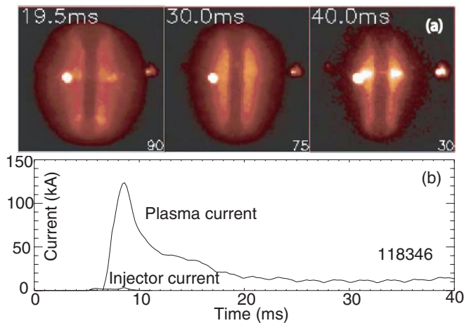
FIG. 4 (color). (a) Shown in the top are fast camera fish eye images during the first 40 ms of a 400 ms discharge. (b) Also shown are I_p and I_{inj} . The small bright image that appears just below and to the left of the plasma ring (in time frame at 40 ms) is light from an electrical filament inside NSTX. The numbers at the bottom of the camera images are maximum scale values for the images.
