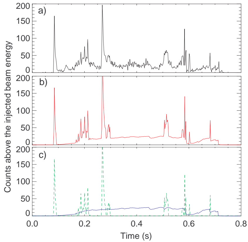
Figure 4. (a) Temporal evolution of counts above the injected beam energy; (b) the empirical linear combination of pulse pile-up and neutron/gamma radiation; and (c) contribution of pulse pile-up (dashed green curve) and neutron/gamma radiation (solid blue curve)
