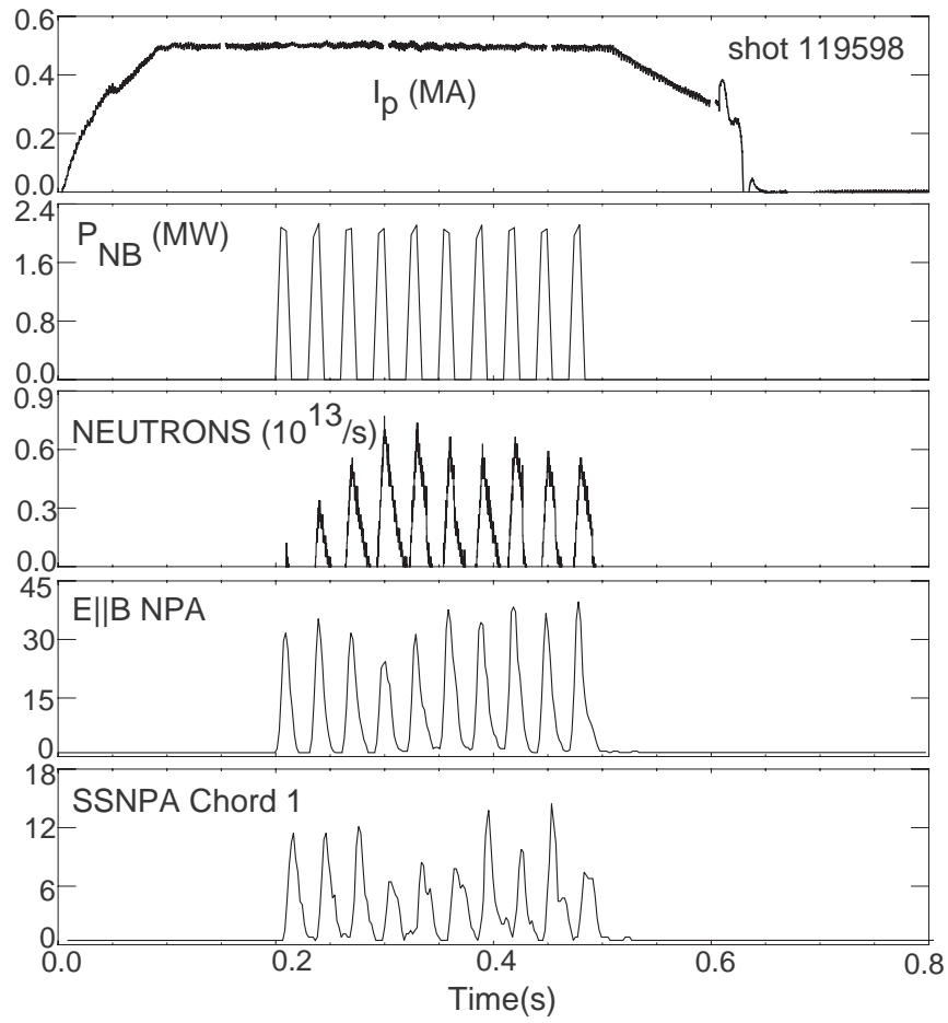
Figure 5. Temporal evolution of plasma current I_p , NB power, neutron yield, counts in chord 1 of the SSNPA (with tangency radius 60cm), and the E||B NPA signal (with tangency radius 63.5cm).
