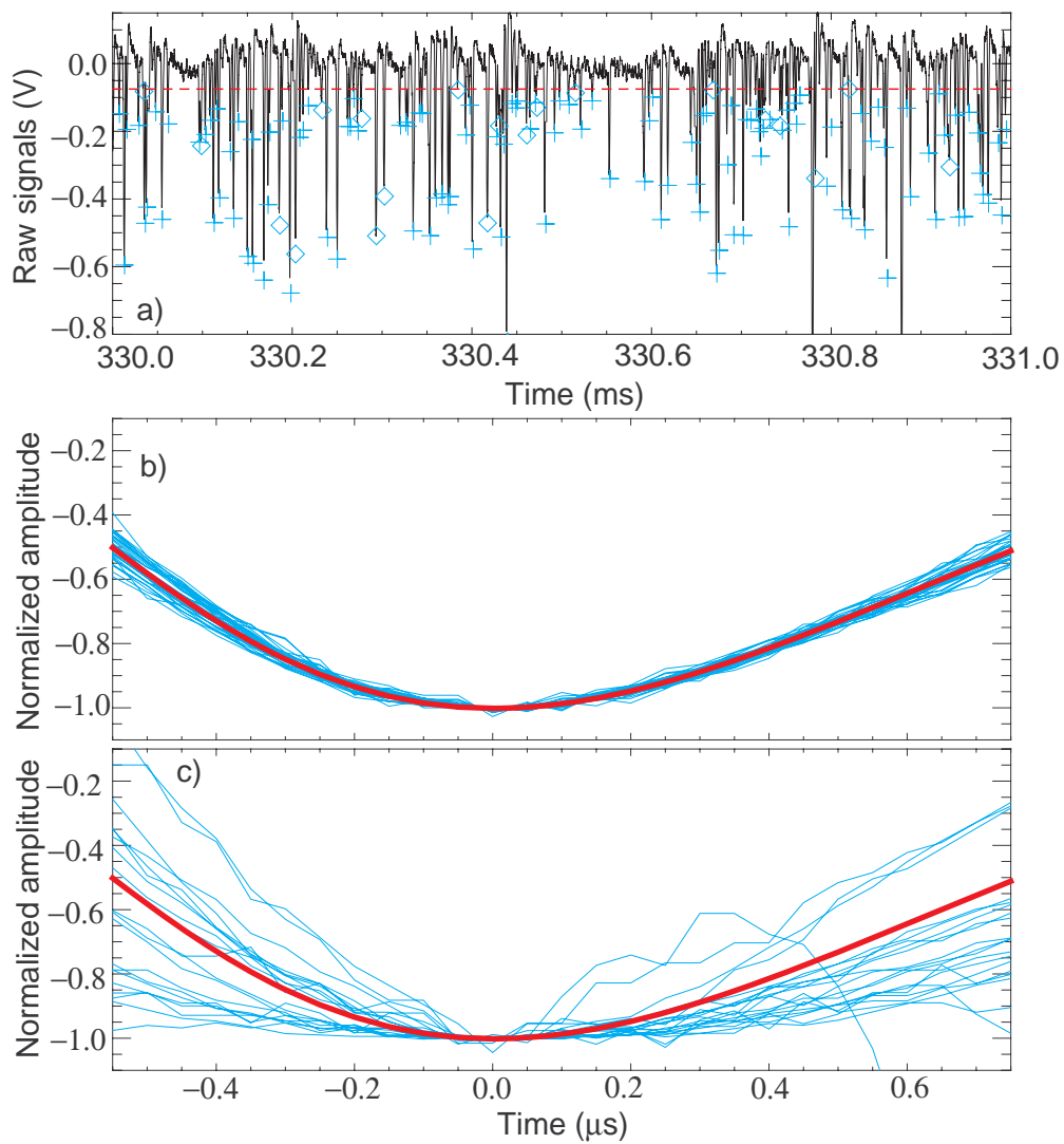
Figure 2. (a) Raw data for chord 1 of the SSNPA with true signals marked with plus and noise marked with diamond; (b) pulse shape comparison of the true signals (solid blue curves) with the pulse model (bold red curve); and (c) pulse shape comparison of noise (solid blue curves) with the pulse model (bold red curve)
