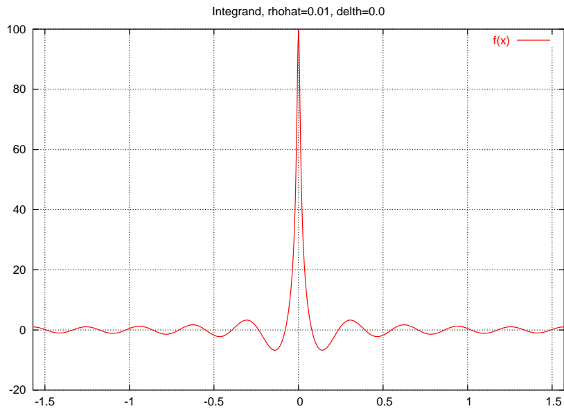
Figure 1: The integrand of \mathcal{G}^n in Eq. (4) with \hat{\rho} = 0.01 and n = 10 .
