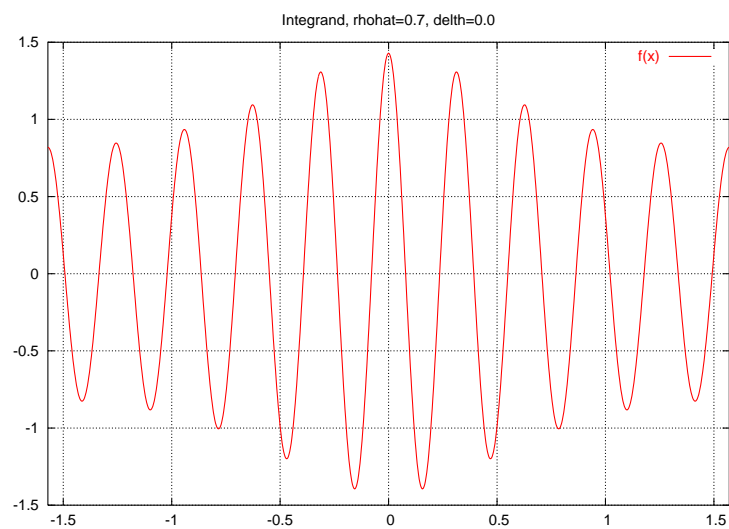
Figure 5: The almost constant amplitude of the integrand of \mathcal{G}^n when \hat{\rho} = 0.7 .
