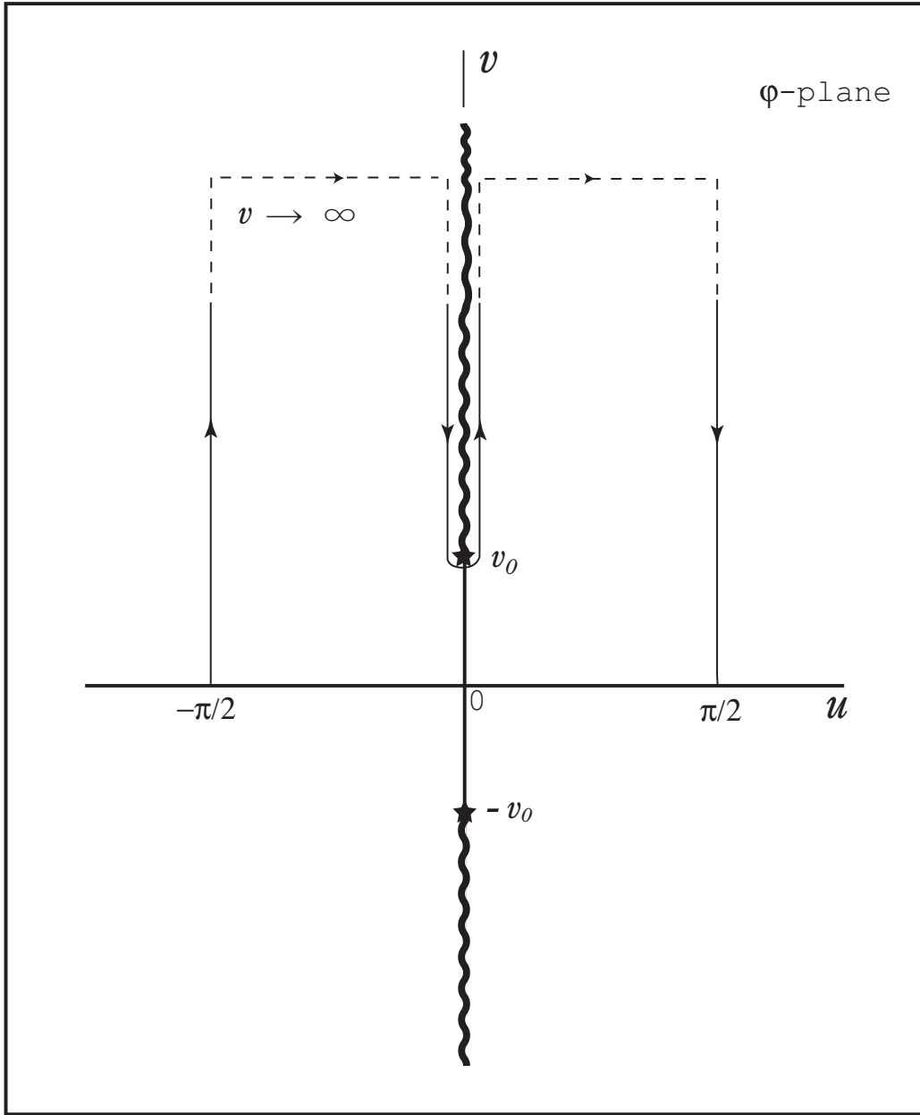
Figure 6: The complex \phi = u + iv plane showing the branch points at v_0 = \pm \sinh^{-1} \hat{\rho} , the corresponding branch cuts denoted by the wavy lines, and the new deformed contour of integration which was originally along the real axis over the range [-\pi/2, +\pi/2] .
