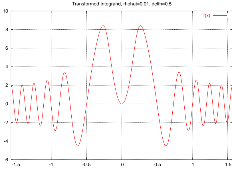
Figure 3: The integrand of \mathcal{G}^n showing the effect of the change of variable \phi' = \phi - \delta \sin 2\phi .
