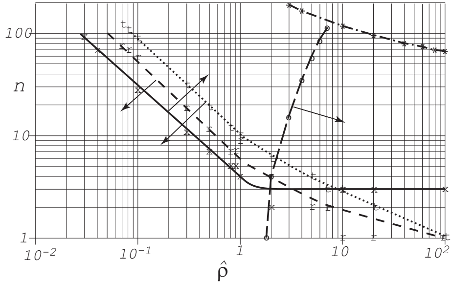
Figure 7: Lines of constant relative error, \varepsilon , in the n vs. \hat{\rho} plane for various algorithms – trapezoidal (dotted line), the recursion (short dashed line), the series expansion (solid line), and the large \hat{\rho} expansion (long dashed line). The arrows indicate the direction where the relative error decreases from 10^{-6} . The dot-dashed line at upper right denotes where the value of the integral approximately approaches the underflow limit, \sim 10^{-300} .
