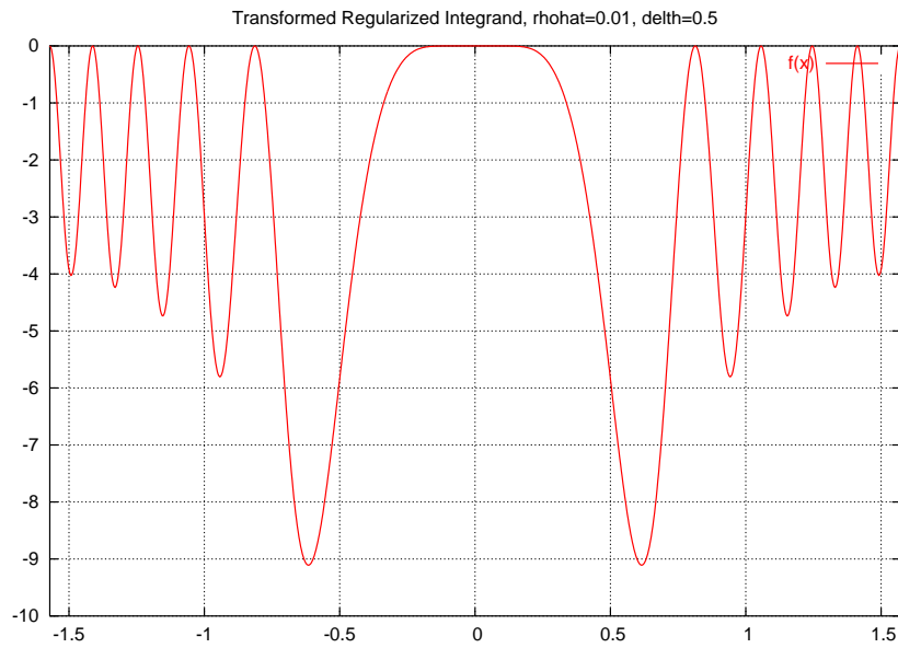
Figure 4: The regularized integrand of \mathcal{G}^n showing the effect of the change of variable \phi' = \phi - \delta \sin 2\phi .
