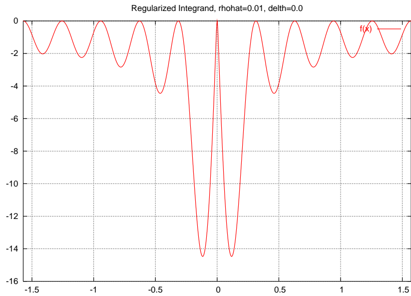
Figure 2: The regularized integrand of Eq. (5) with \hat{\rho} = 0.01 and n = 10 .
