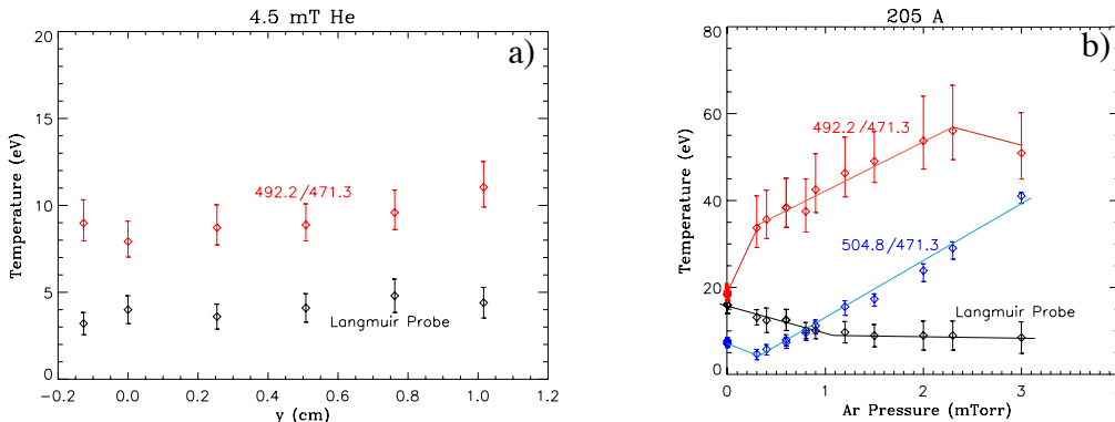
Figure 11: a) Radial profiles of T_e determined by the Sasaki et al. [34] collisional-radiative model and with the Langmuir probe. b) The dependence of three calculated electron temperatures, using probe data and the Sasaki method, on argon fill pressure in a helium helicon discharge.
