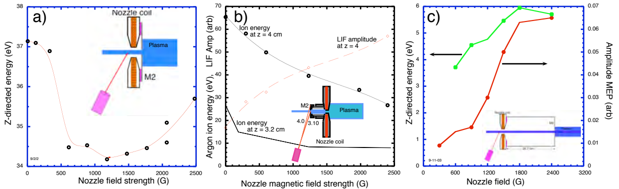
Figure 5: a) E_z of the HEP ions versus nozzle-field strength at z = 2 \text{ cm} in the ER. The plate M2 was located 1 cm upstream of the nozzle coil midplane, as shown in the inset. b) HEP E_z versus nozzle-field strength at z = 3.2 and 4.0 \text{ cm} from the nozzle-coil midplane. M2 was located 3.1 cm downstream of the nozzle-coil midplane, see inset. c) E_z of the MEP ions versus nozzle field strength at z = 2 \text{ cm} from the nozzle-coil midplane. M2 was located 26.7 cm upstream of the nozzle-coil midplane, see inset.
