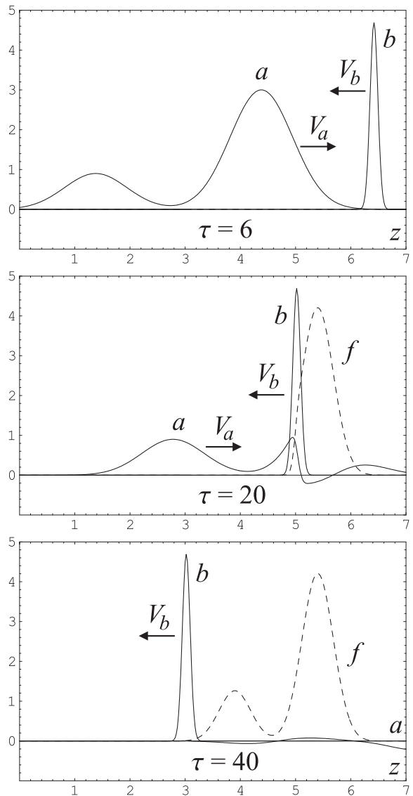
FIG. 4: Raman interaction between an optical pulse a and a counter-propagating reference pulse b with \epsilon_{\text{rec}} = \pi/2 (arbitrary units). Electromagnetic pulse a is almost fully depleted after the interaction; the electrostatic wave has a maximum possible amplitude
