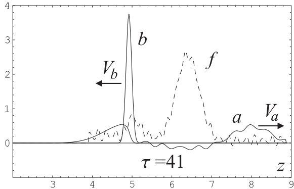
FIG. 6: Recording an optical pulse a into a noisy Raman medium by a counter-propagating reference pulse b (arbitrary units). Thermal oscillations f_n existing in the Raman medium are added to the desired profile of the electrostatic wave f (dashed)
