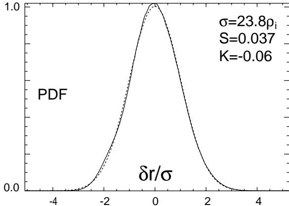
FIG. 2. Probability density function of test particle radial displacement (solid line) is very close to a Gaussian (dotted line). \sigma , S , K are, respectively, the standard deviation, skewness, and kurtosis of the measured data.
