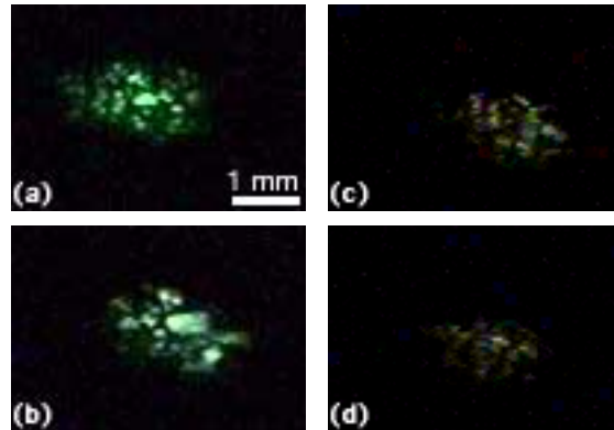
Fig. 10 Still images from a video taken of the Nd laser interacting with the surface of KC17 cube 2B. The laser power was 80 \text{ W/mm}^2 , atmosphere argon, and the scan was in the horizontal direction at a speed of 50 \text{ mm/s} . Frames (a) and (b) are from the left, light gray area as seen in fig. 6; frames (c) and (d) are from the blacker area on the right. The light emission was attenuated by \times 100,000 with a neutral density filter. Micro ‘hot spots’ are evident. The scale bar in (a) applies to all frames.
