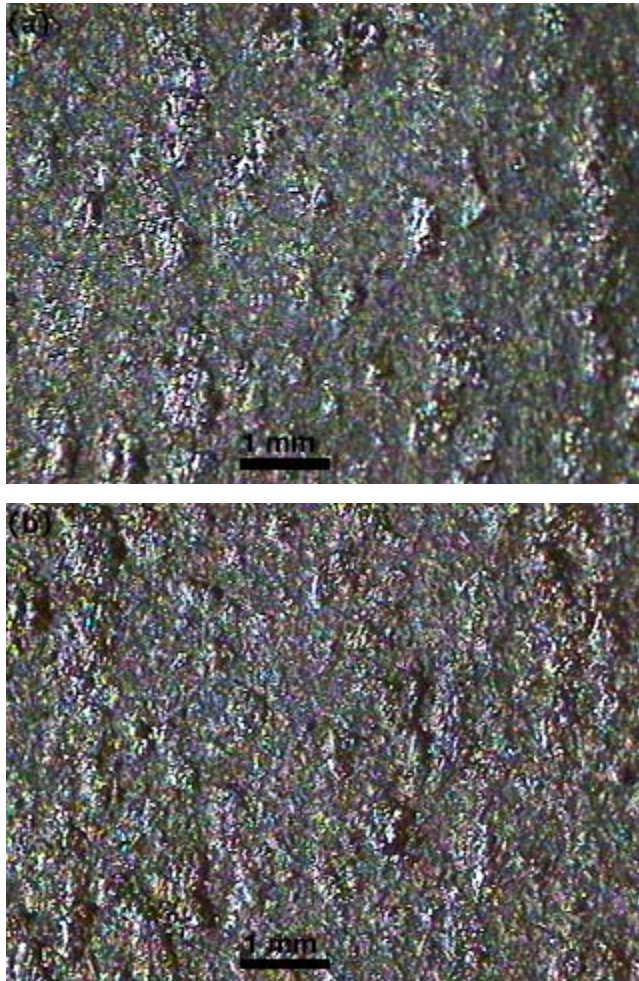
Fig. 9 Microscope images taken normal to the surface of KC17 cube 6E surface before (a) and after (b) a Nd laser scan ( 80 \text{ W/mm}^2 , 1000 \text{ mm/s} ). At this high scan speed there is very little difference in the appearance even though the surface was heated to 1770 \text{ C} (fig. 5) by the laser and 18 \text{ mCi} of tritium released.
