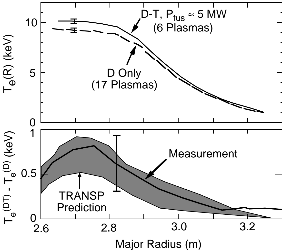
Fig. 5. Comparison of the electron temperature profile for a set of similar D-T and D discharges with comparable energy confinement times and neutral-beam heating power. The measured difference in electron temperature is consistent with the predicted change due to alpha heating. (Taylor et al. 1996)
