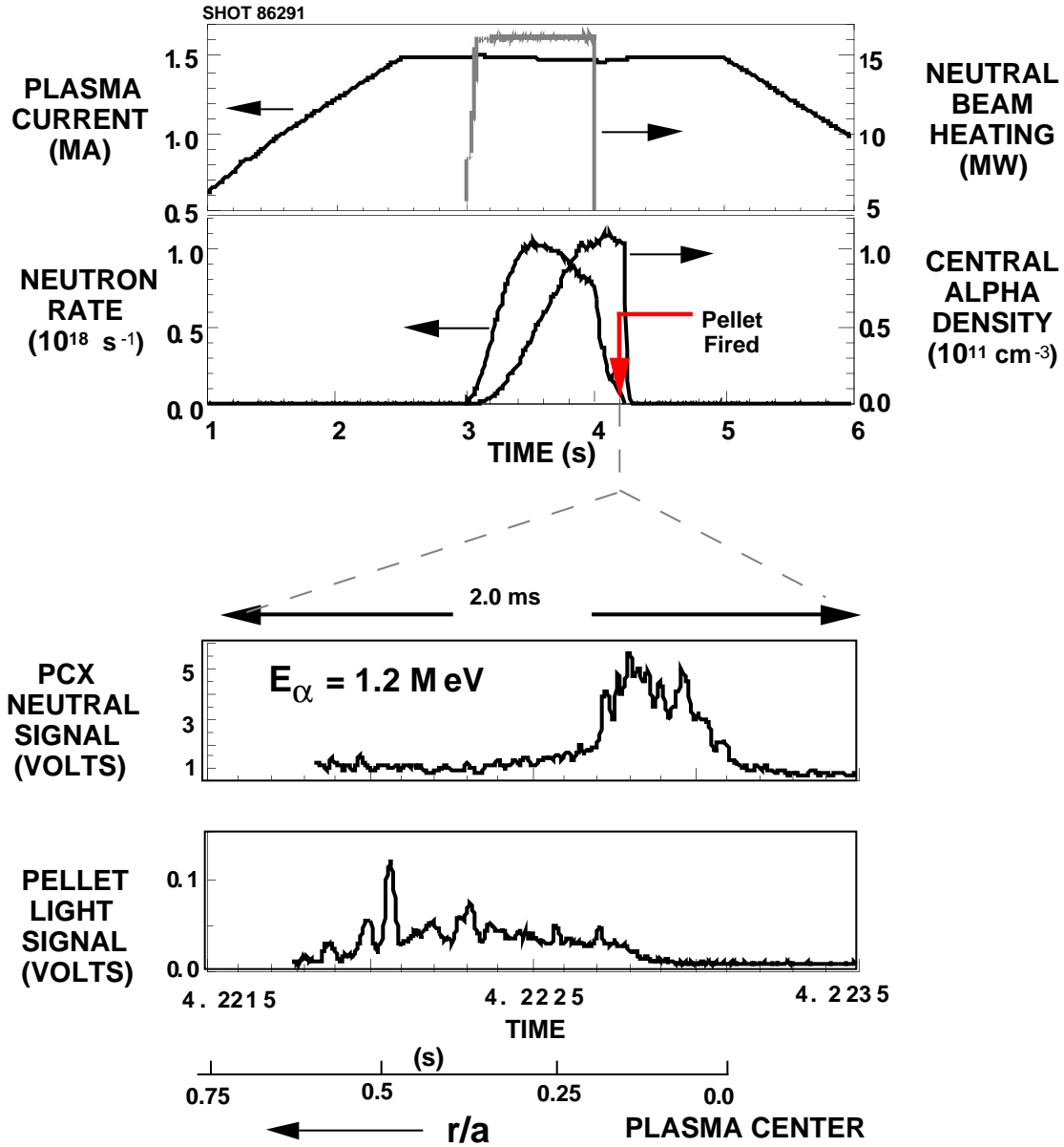
Fig. 5 Selected plasma waveforms and PCX signals for measurement of the alpha spectrum up to the birth energy using single boron pellet injection.
