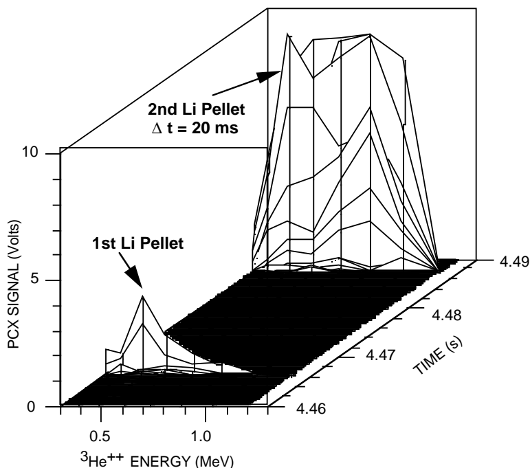
Fig. 19 Illustration of the enhanced PCX {}^3\text{He}^{++} signal for the second pellet using "stacked" lithium pellet injection (same TFTR discharge as in Fig. 18).
