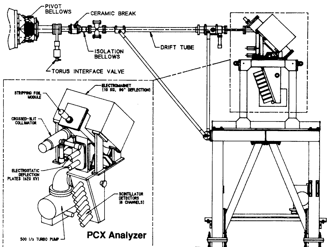
Fig. 2 Schematic of the Pellet Charge Exchange (PCX) diagnostic installed on TFTR.
