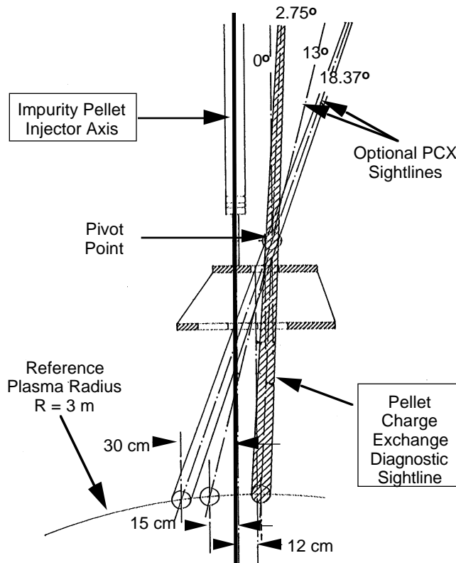
Fig. 4 Field-of-view of the Pellet Charge Exchange (PCX) diagnostic relative to the pellet flight path of the Impurity Pellet Injector (IPI). The PCX apparatus is currently installed at the 2.75° position.
