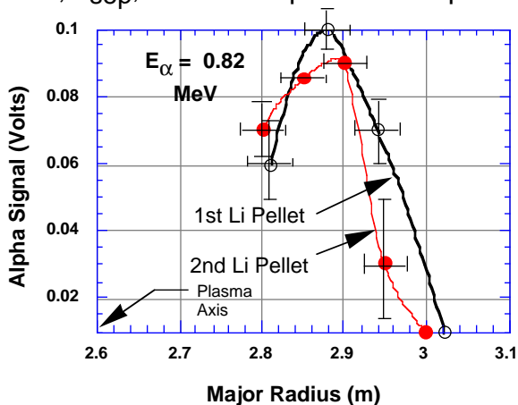
Fig. 20 Example of alpha density profile measurements using stacked pellets.
