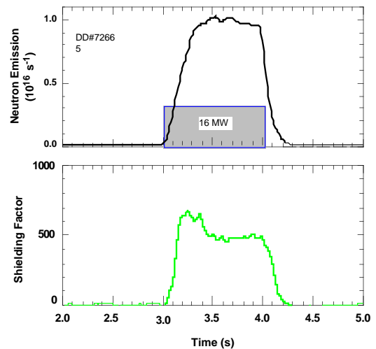
Fig. 6 For a D-D plasma, the measured shielding factor is ~ 500.
