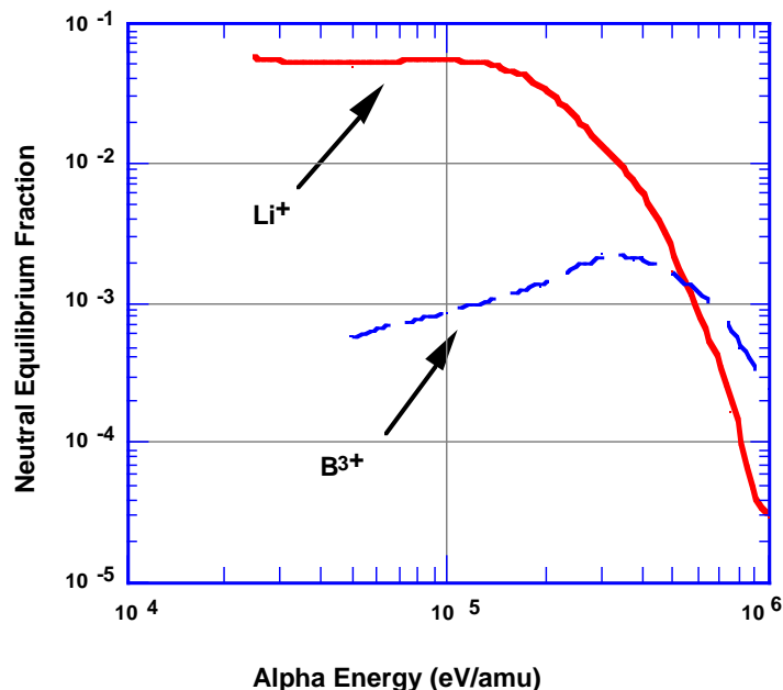
Fig. 14 Calculated neutral equilibrium fractions for \alpha -particles on Li^+ and B^{3+} targets.
