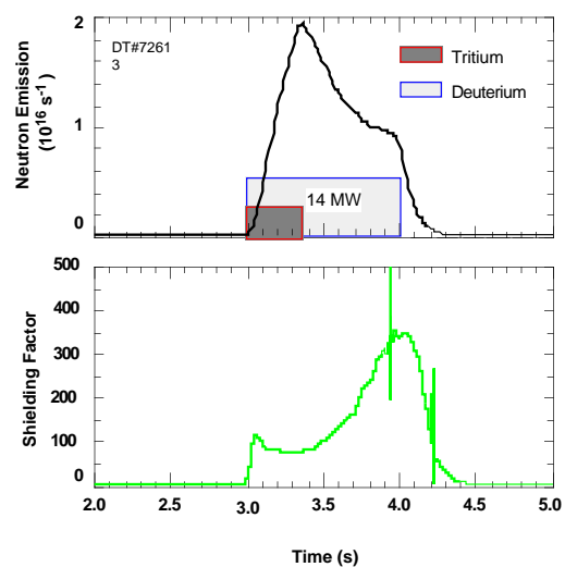
Fig. 7 For a D-T plasma, the measured shielding factor is ~ 100
