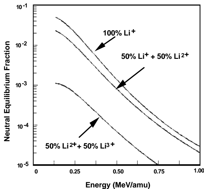
Fig. 15 Illustration of the effect of lithium ionization state mix on the computed neutral equilibrium fractions for alpha particles .
