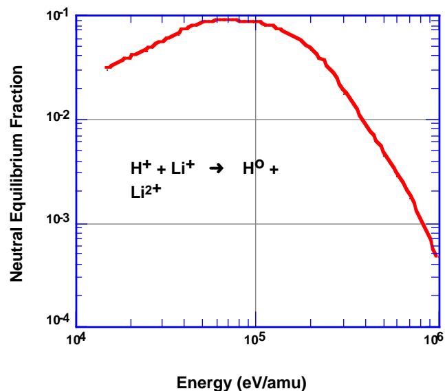
Fig. 16 Computed equilibrium fractions for H^+ (or D^+ , T^+ ) ions on a Li^+ target.
