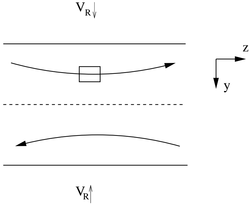
FIG. 1: The small region around the X line.
