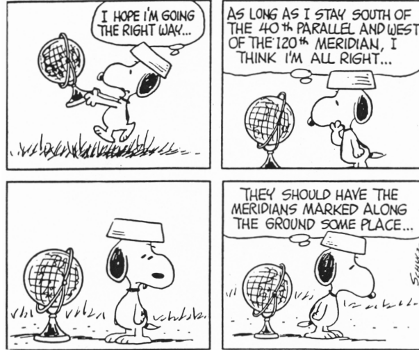
FIGURE 5. Quest of useful coordinates [40]. (Peanuts by Charles Schulz. Reprint permitted by UFS, Inc.)
