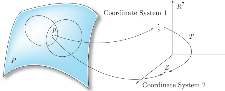
FIGURE 4. Coordinate transformation as a map in R^7 .
