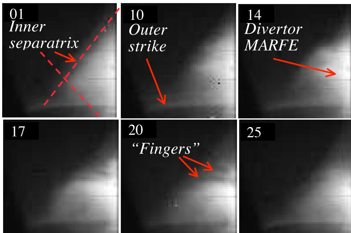
Fig. 8 – divertor camera images of unfiltered light during a Type V ELM (#112503 @ 0.398 sec). The relative frame numbers are indicated and the time between frames is 24.7 \mu sec. The perturbation persists for ~ 400 \mu sec.
