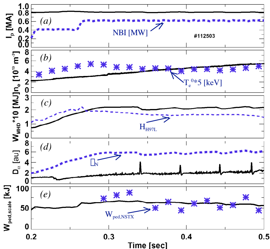
Fig. 1 – Example of a Type I ELMy discharge: (a) I_p and P_{NBI} , (b) \bar{n}_e and central T_e , (c) stored energy ( W_{MHD} ) and confinement relative to ITER-97 L-mode scaling ( H_{H97L} ), (d) D_\alpha and \square_N , and (e) comparison of pedestal stored energy (blue data points) with an international scaling. Panel (e) is discussed in section II.
