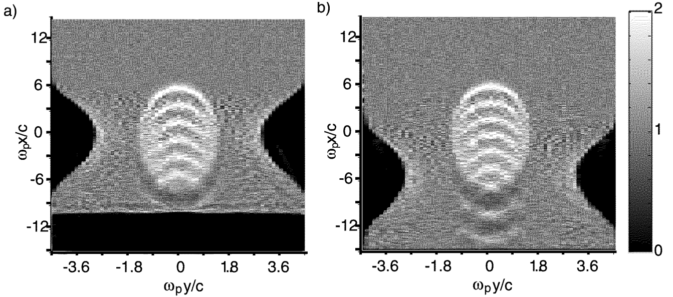
Figure 3. Beam entry into the background plasma for the same conditions as in Fig.1 but at later times. Figure 3(a) is taken at a time interval 3\pi/\omega_p later than Fig. 1(d), and Fig. 3(b) is taken at a time interval 30\pi/\omega_p later than Fig. 3(a). Note that the hole velocity in the beam frame is approximately 6c/30\pi \approx c/16 or 1/8^{\text{th}} of the beam velocity.
